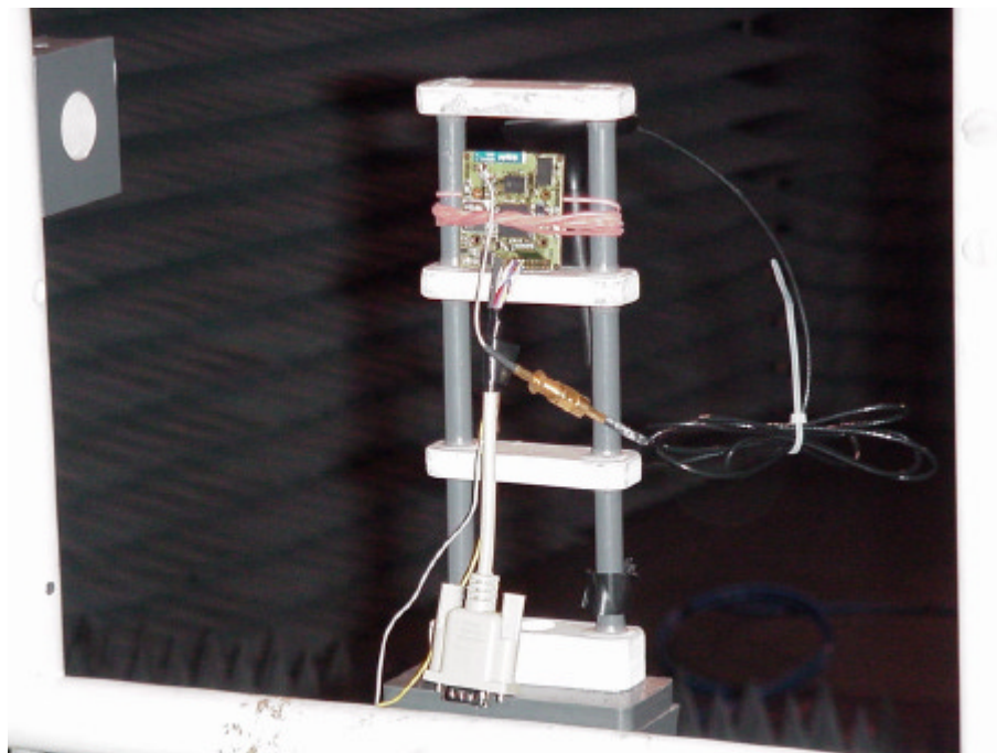
Picture 4 : Setup for radiated emission tests, close-up
