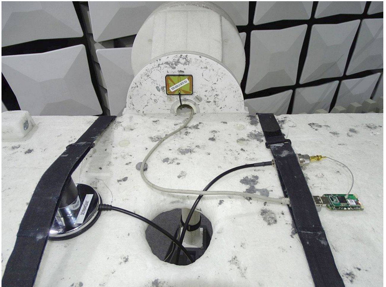
Photo 2: Detail of the test setup on turn unit
