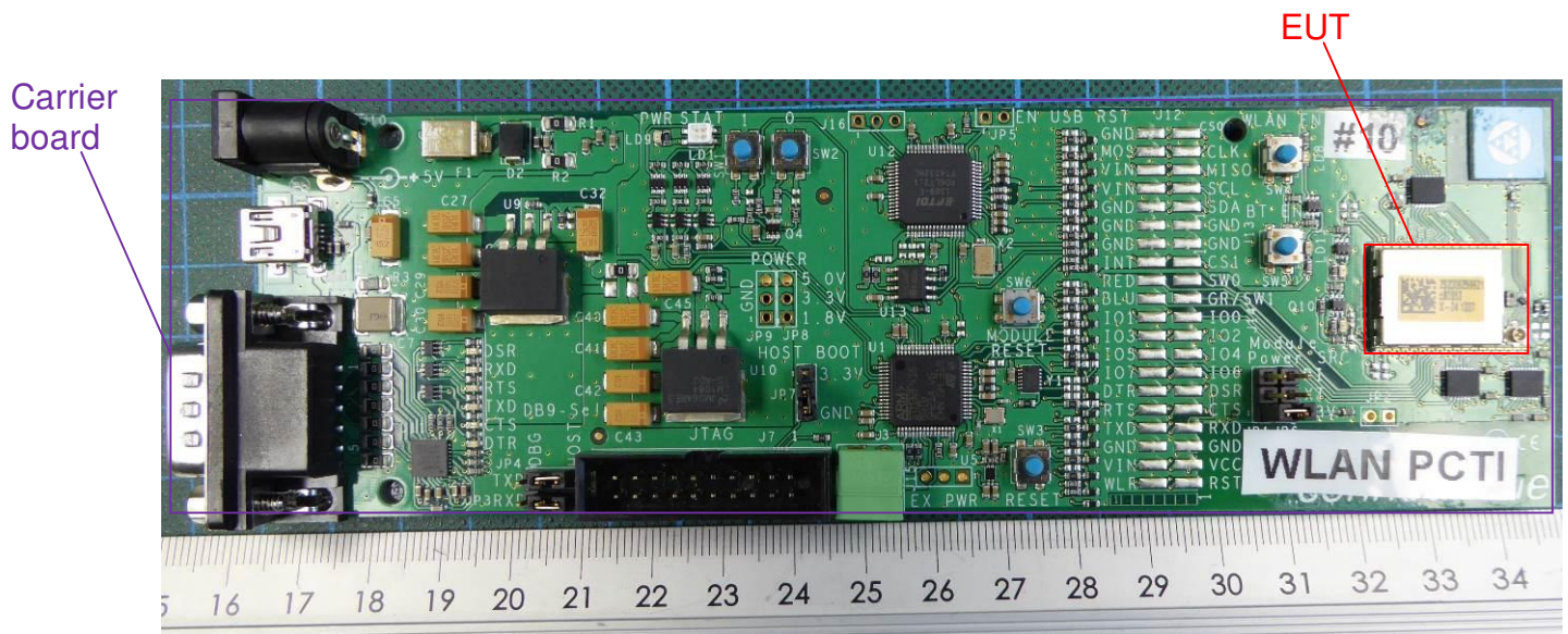
160912_2.jpg: EUT + test PCB – top view
