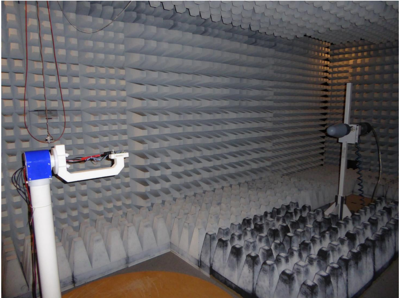
161944_TS031.jpg: Test setup fully anechoic chamber Measurement form 4 to 12 GHz
