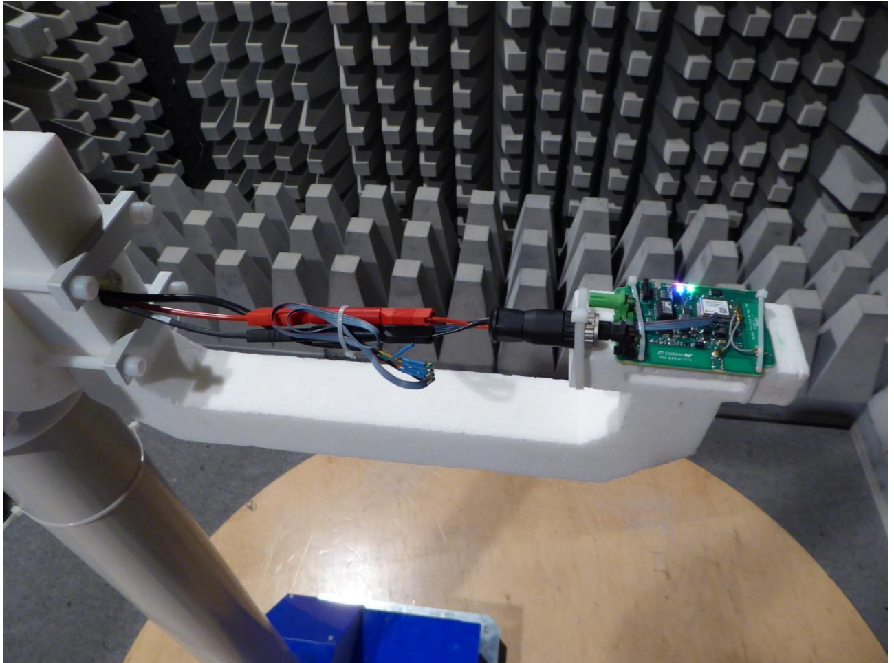
161944_TS001.jpg: Test setup Detail view of EUT on positioner
