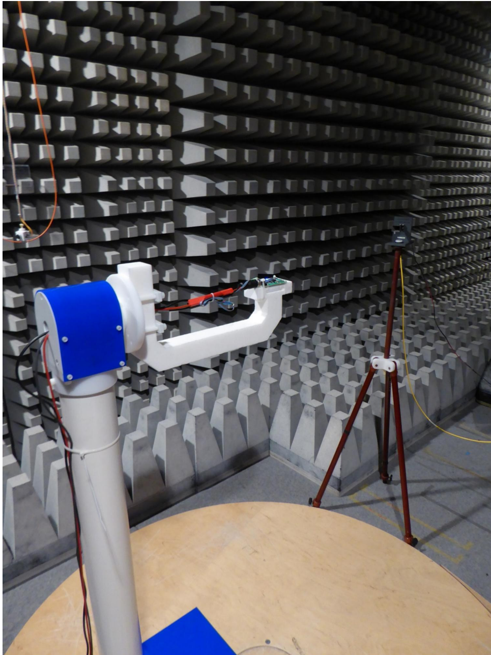
161944_TS020.jpg: Test setup fully anechoic chamber Measurement form 26.5 – 40 GHz (15.407 only)
