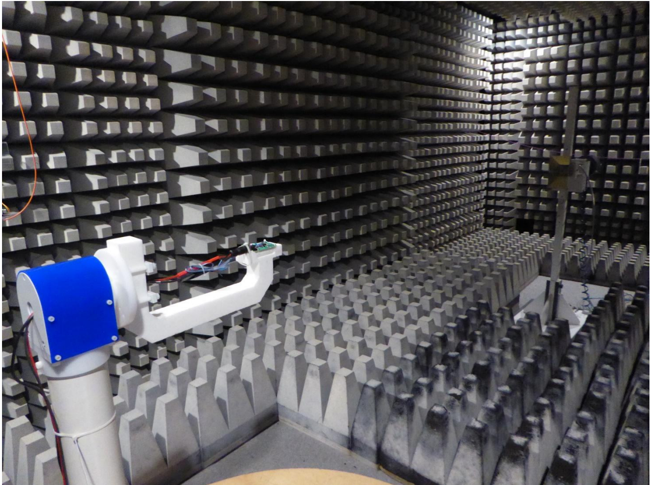
161944_TS004.jpg: Test setup fully anechoic chamber Measurement form 1 to 4 GHz
