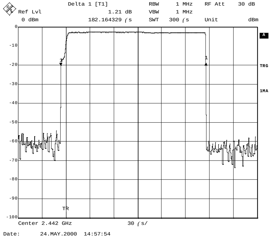
Figure 6: 300 microsecond plot of activity on one channel in page mode
