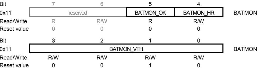
Figure 9-13. Register BATMON.
