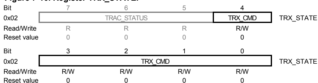
Figure 7-10. Register TRX_STATE.
