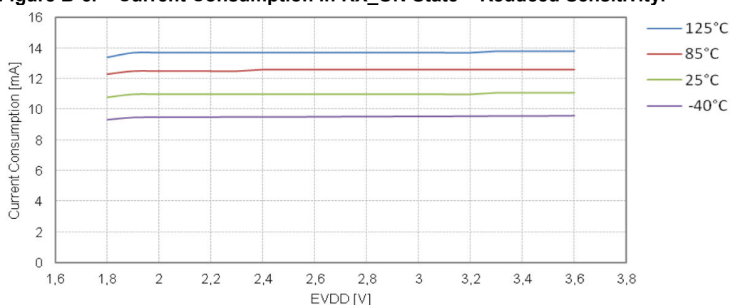
Figure B-6. Current Consumption in RX_ON State – Reduced Sensitivity.
