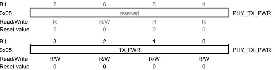
Figure 9-6. Register PHY_TX_PWR.
