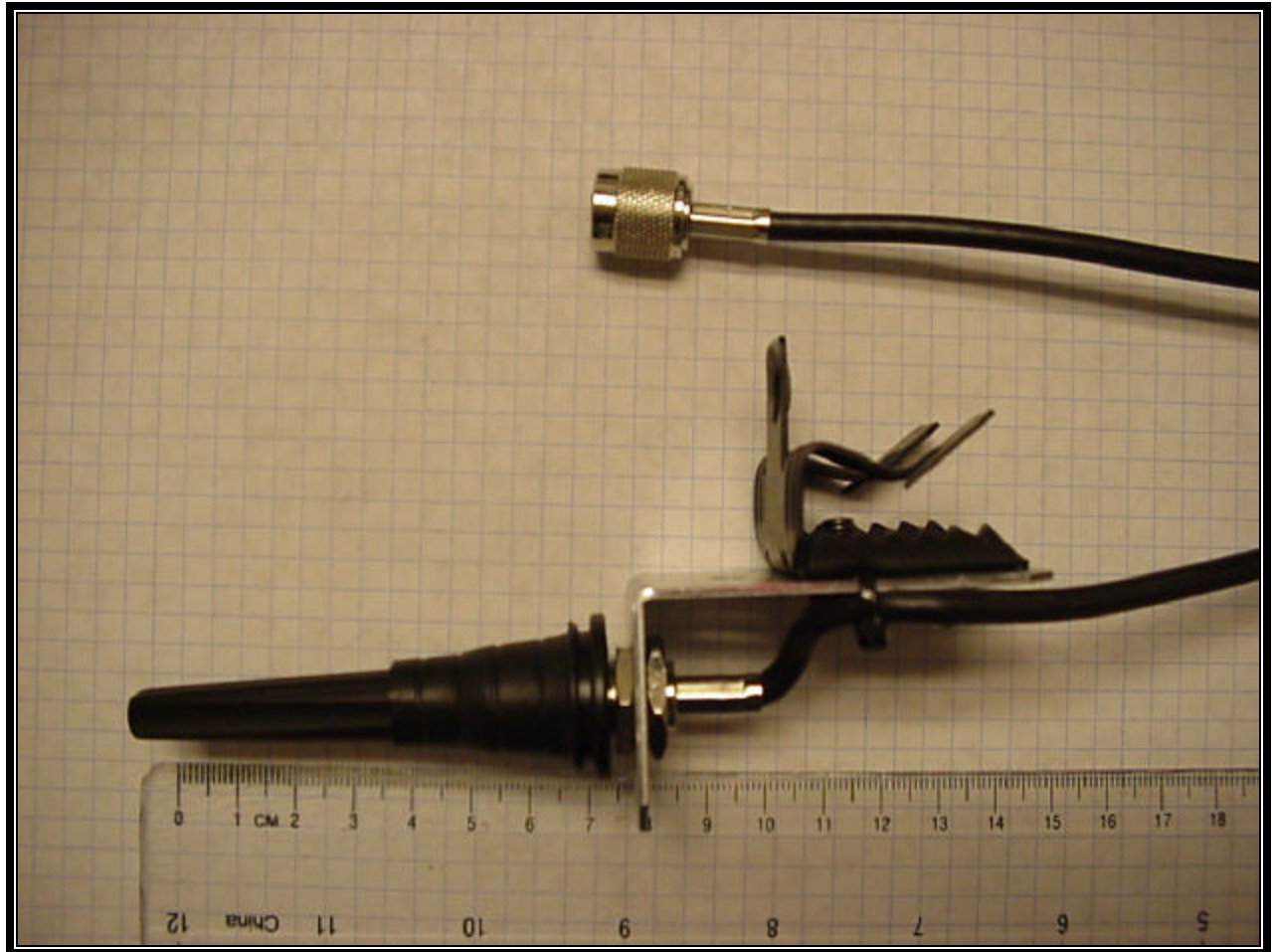
Photograph 6: Antenna Attached to Mounting Bracket/Cable Configuration
