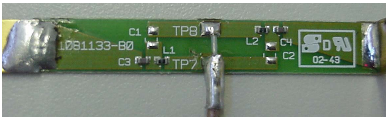
Figure 23 PCB internal antenna TR800
