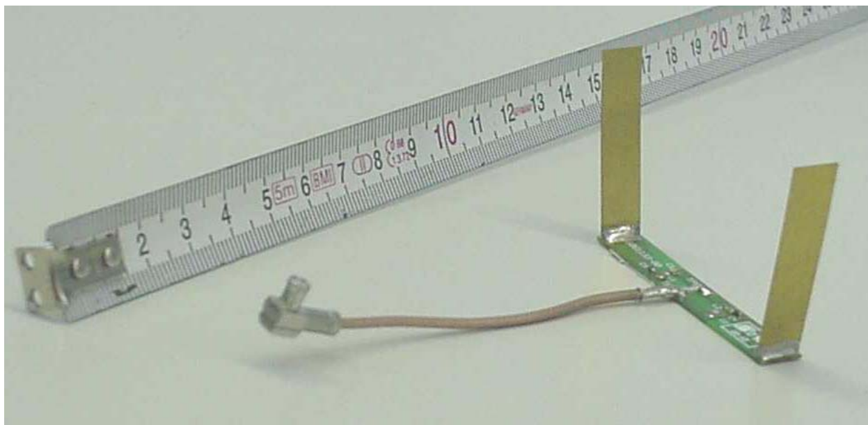
Figure 20 Internal Antenna Model AKT_S (S/N 2303719)
