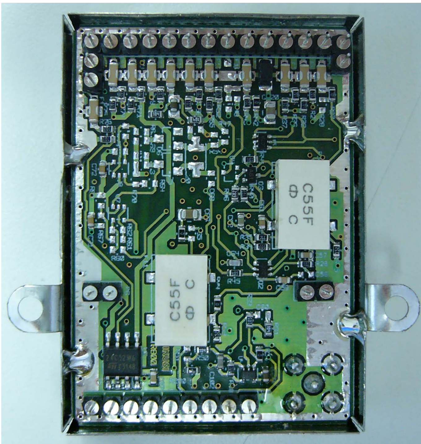
Figure 19 TR800-US. Bottom View Picture
