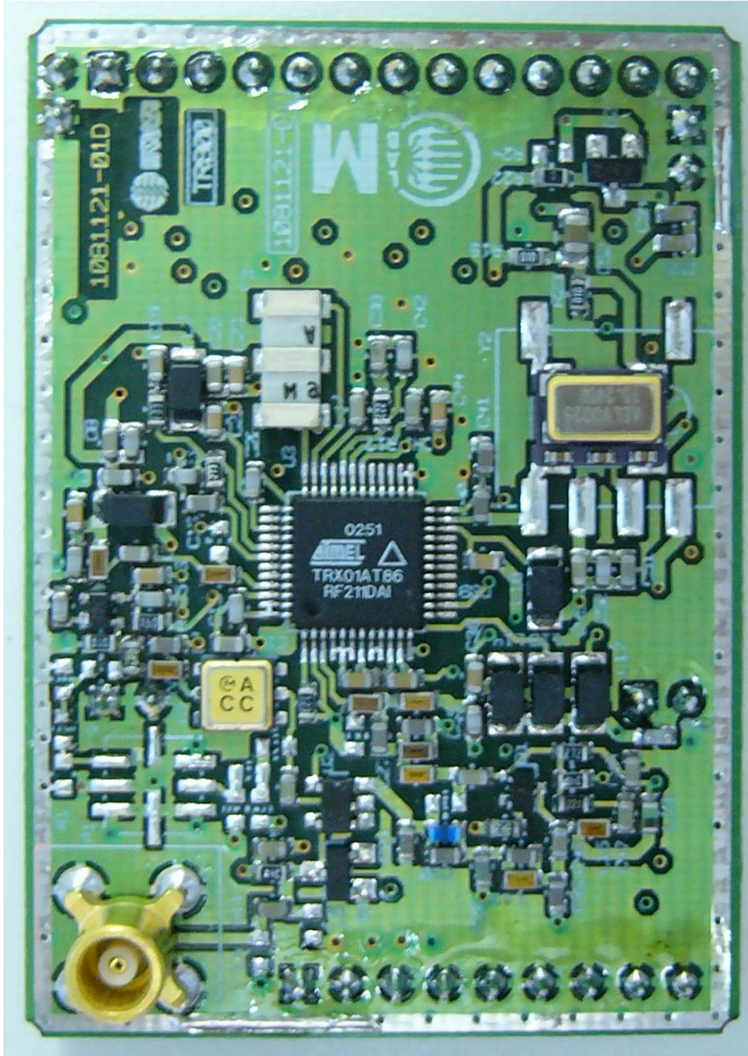
Figure 18 TR800-US. Unshielded Top View
