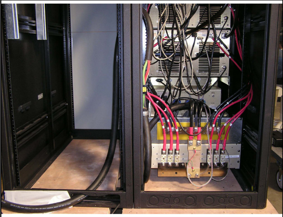
Rear Cabinet Bottom Third
