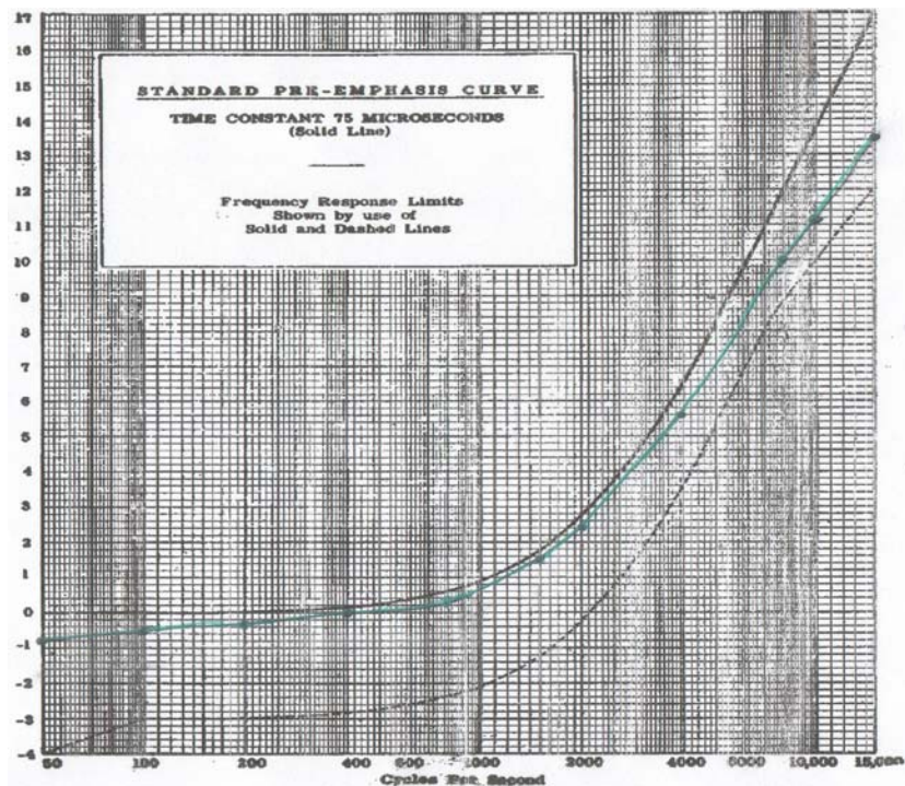
AURAL FREQUENCY RESPONSE GRAPH WITH LIMITS
