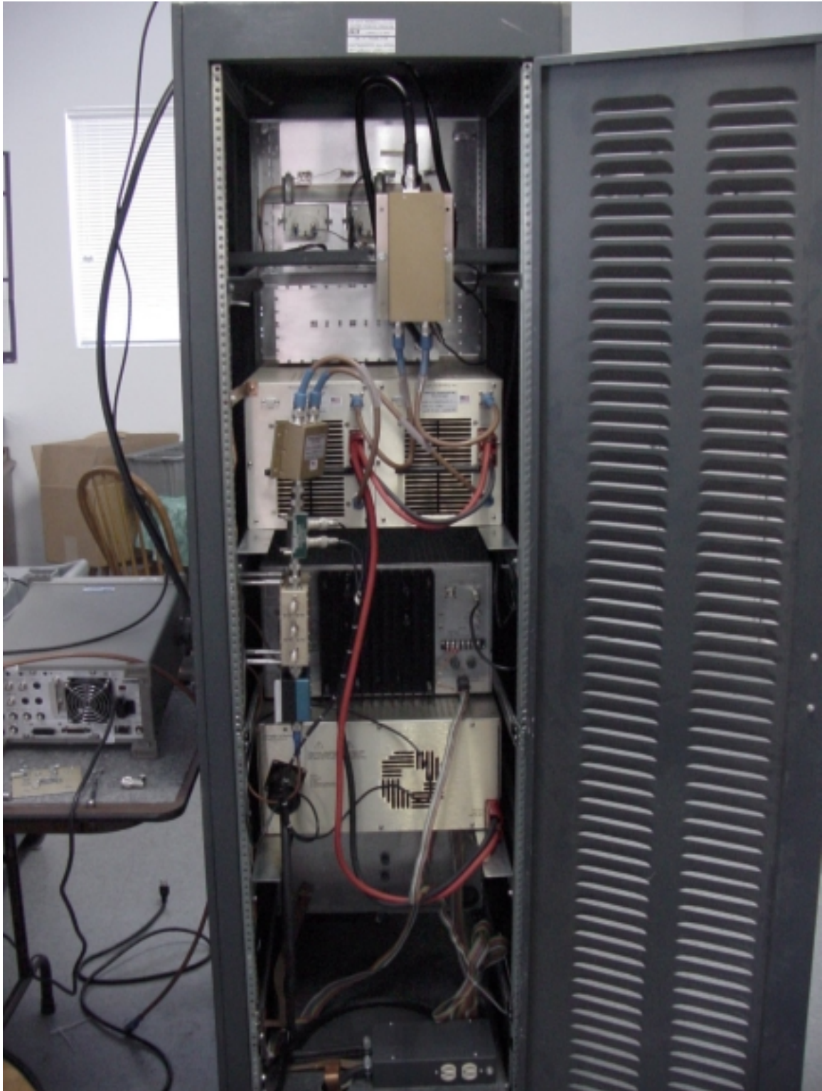
CABINET REAR VIEW WITH DOOR OPEN
