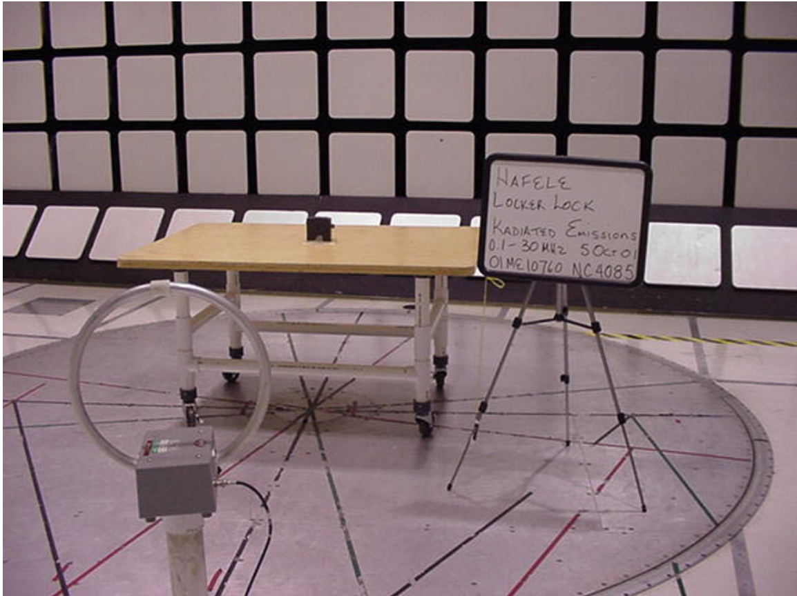
Radiated Emissions Test 0.1 – 30MHz
