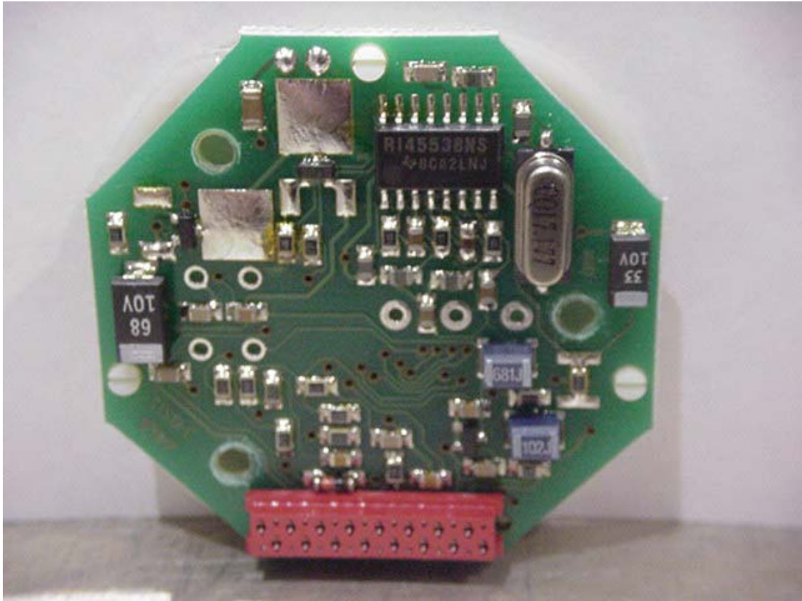
STS-13 Reader PCB
