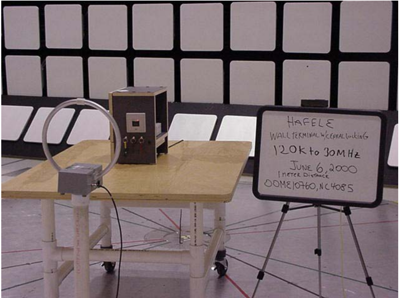
Radiated Emissions Test .1 – 30 MHz
