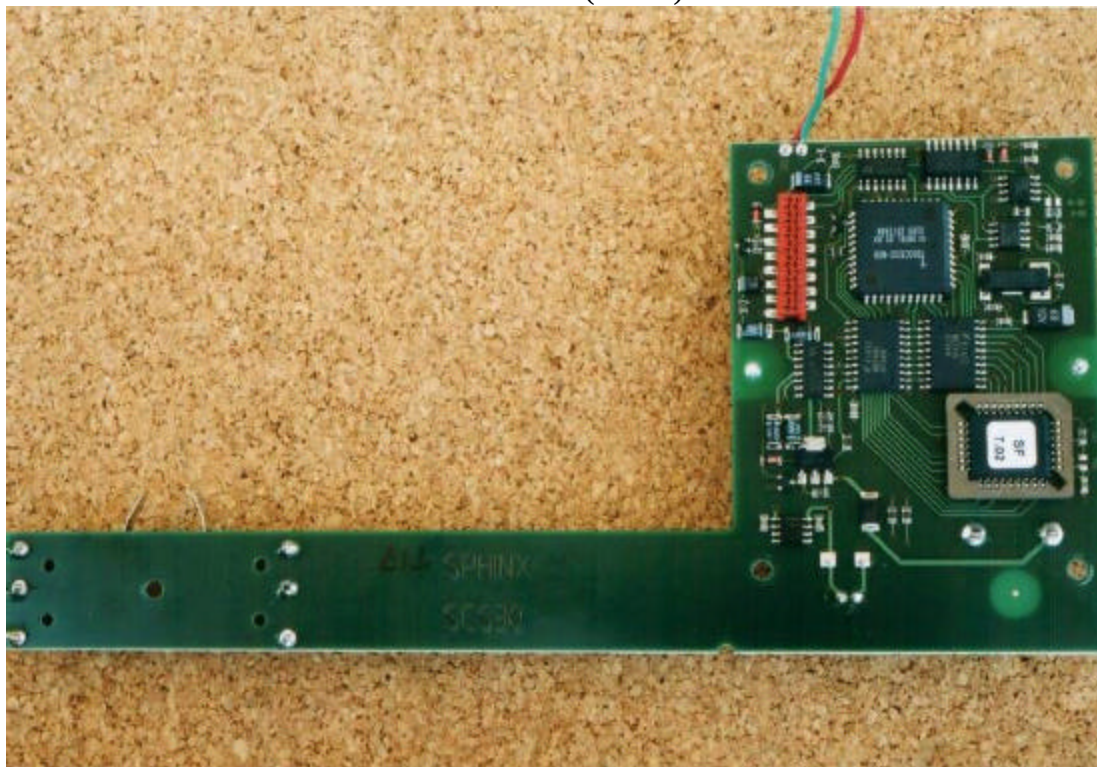
DMT 32 (TIRIS) – Internal PCB & Lock Mechanism
