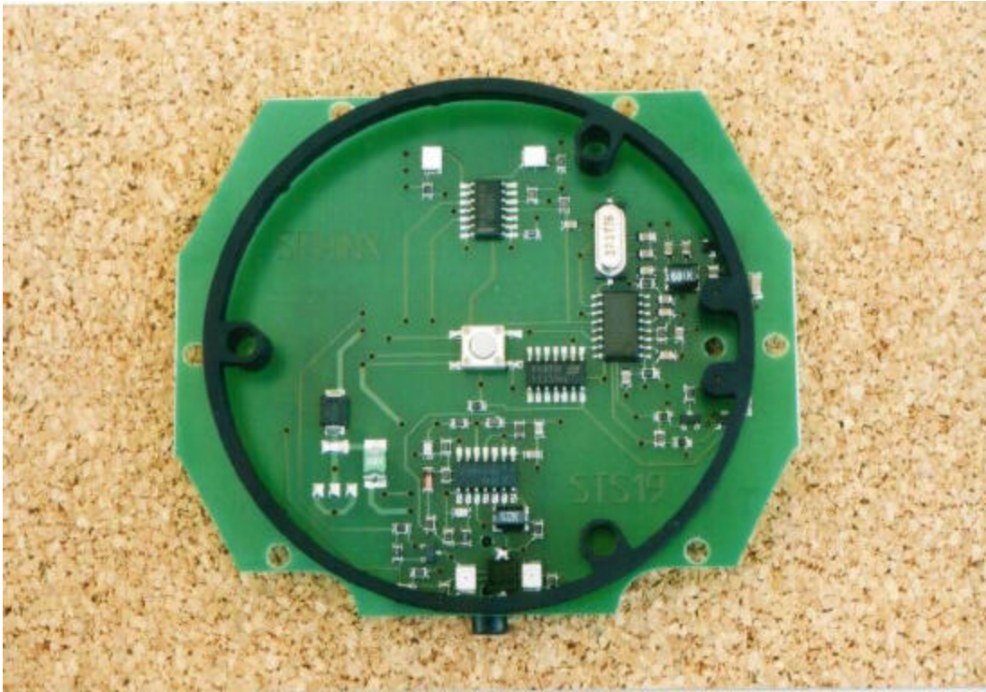
DMT 32 (TIRIS) PCB Front with Coil
