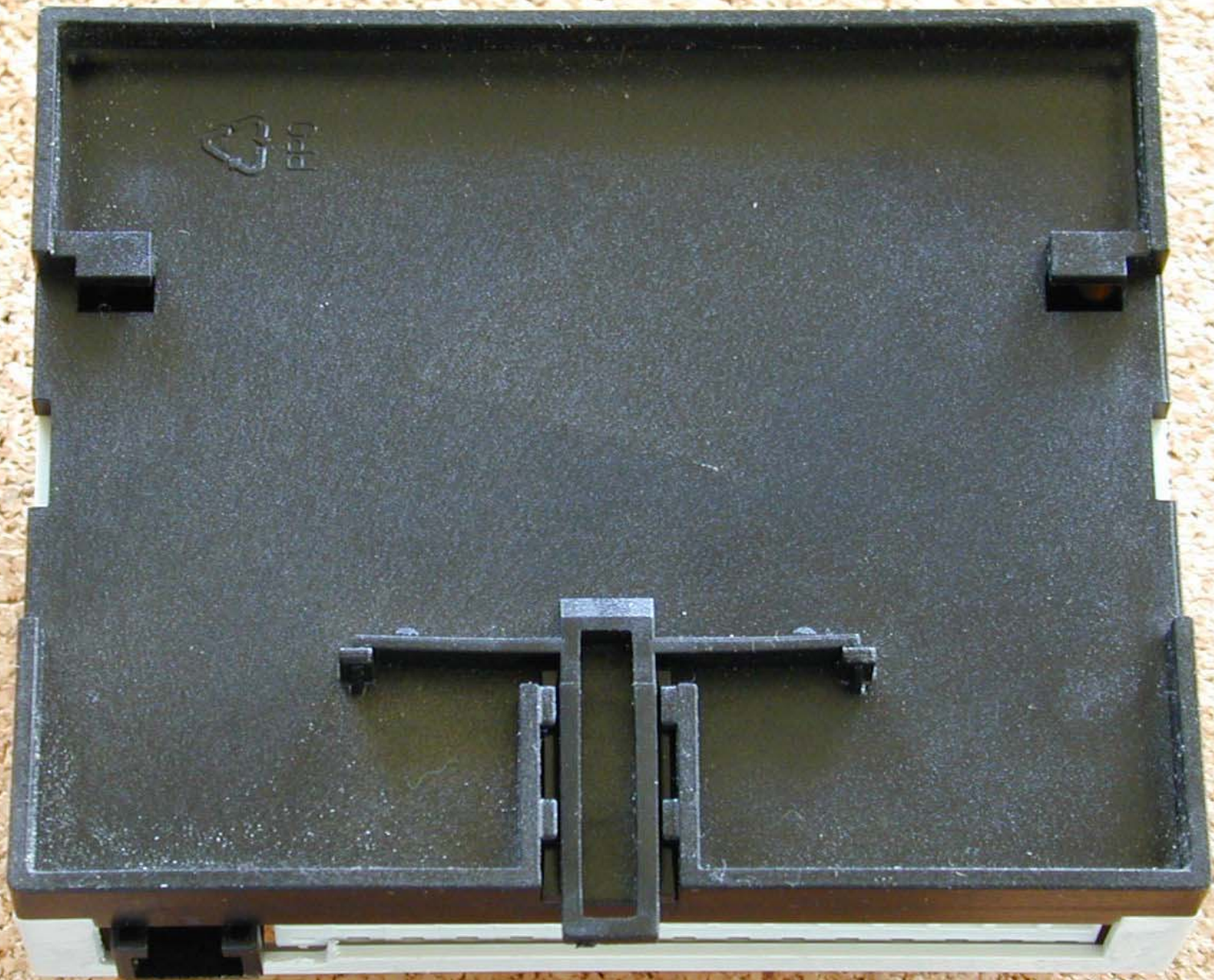
WT2000T Control Box (bottom)
