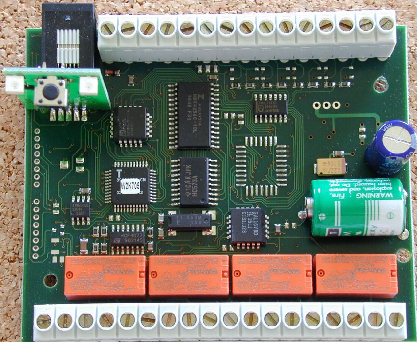
WT2000T Contol Box PCB (top)
