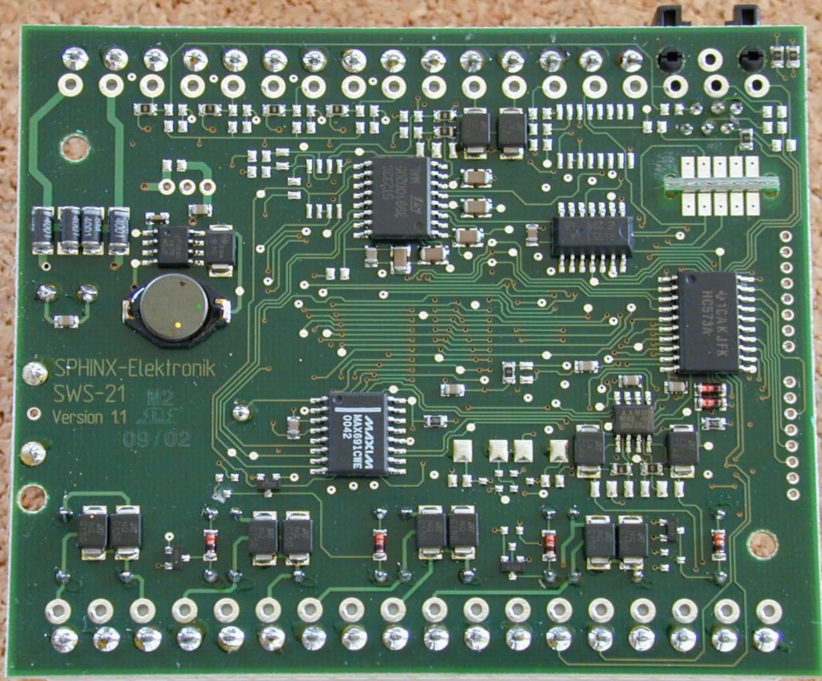
WT2000T Control Box PCB (bottom)
