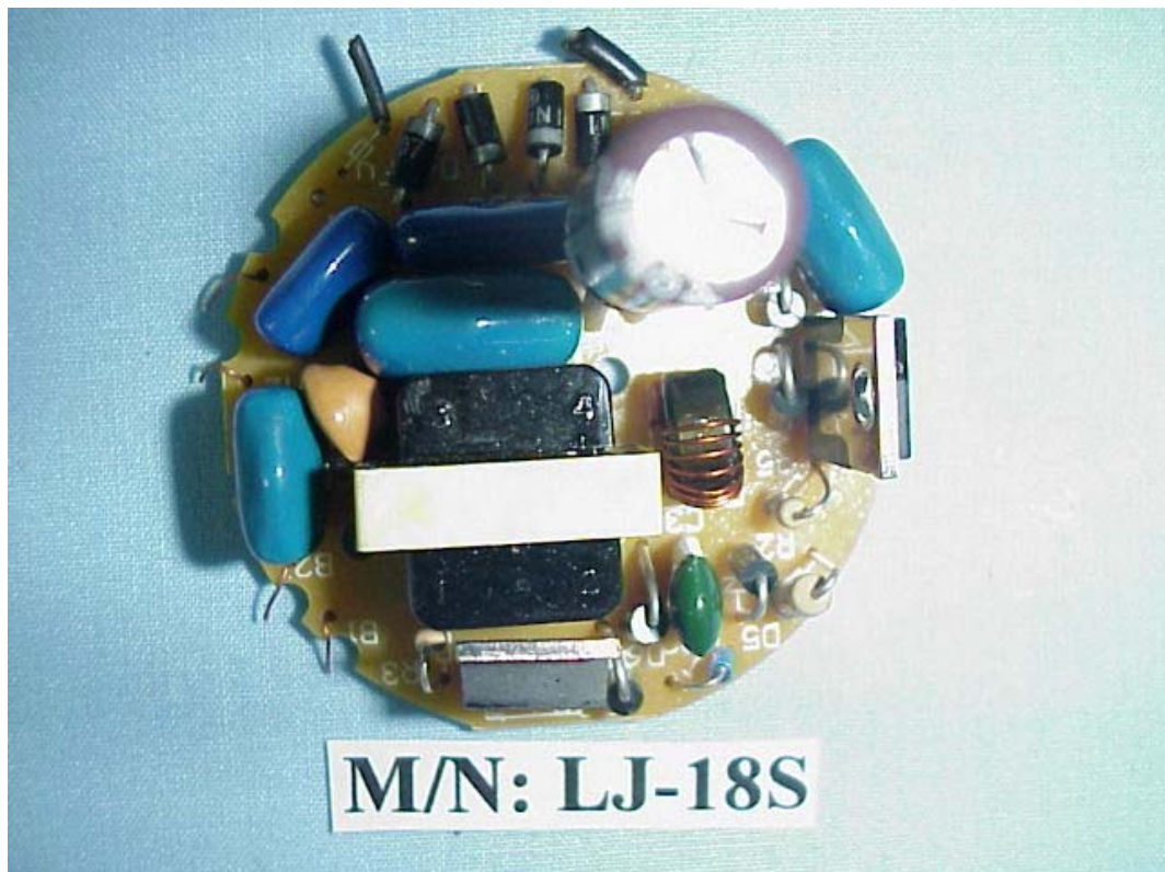
FIGURE 8 ENERGY SAVING LAMP (M/N: LJ-18S) MAIN BOARD (COMPONENT SIDE)
