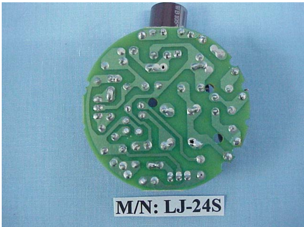
FIGURE 3 ENERGY SAVING LAMP (M/N: LJ-24S) MAIN BOARD (SOLDERED SIDE)
