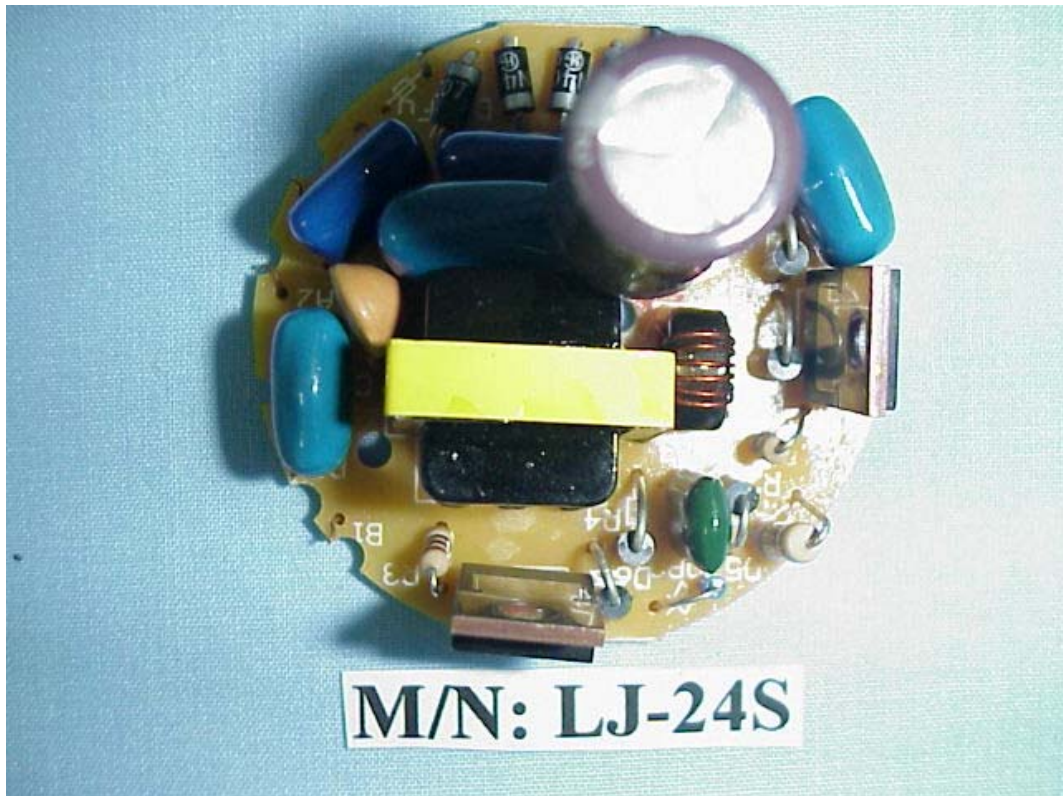
FIGURE 2 ENERGY SAVING LAMP (M/N: LJ-24S) MAIN BOARD (COMPONENT SIDE)
