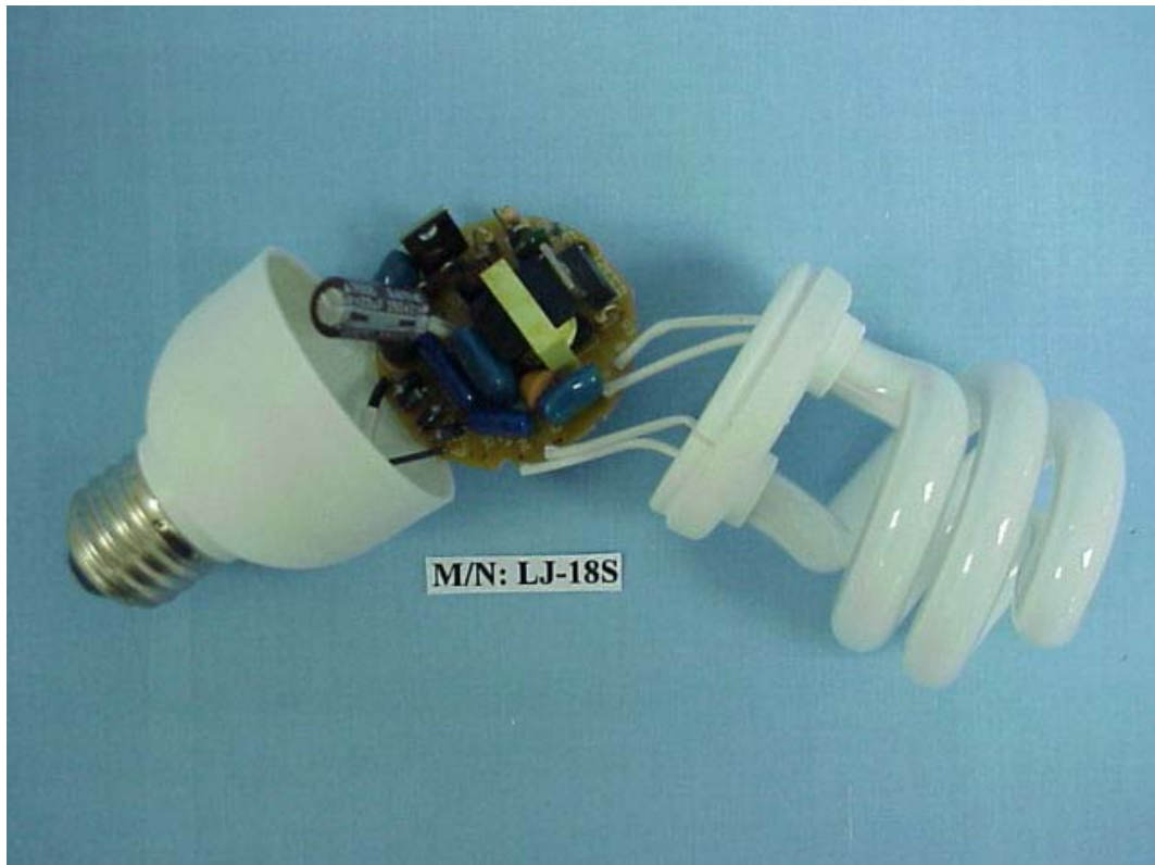
FIGURE 7 ENERGY SAVING LAMP (M/N: LJ-18S) COVER REMOVED
