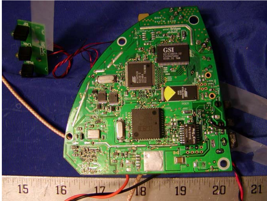
Main Board - Solder View I
