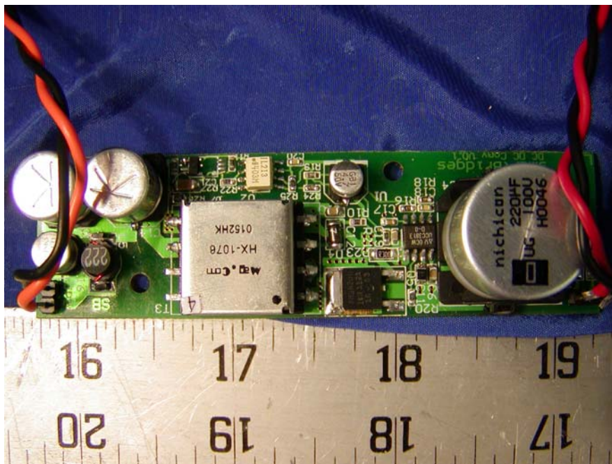
Main Board - Component View II
