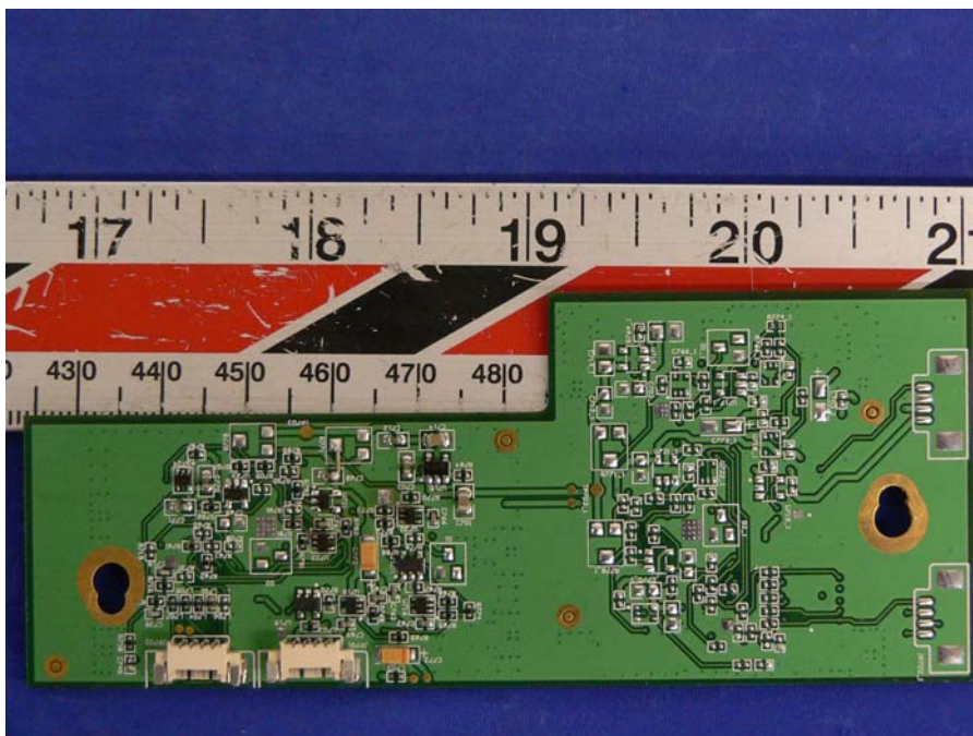
Board 2 Bottom View
