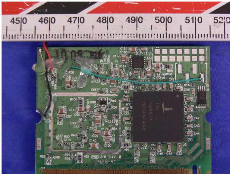
Board 1 Bottom View
