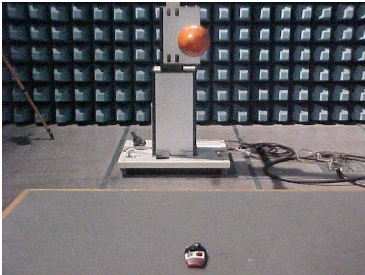
PHOTO N°3 – SET-UP EMISSION TESTS (SPURIUS)
