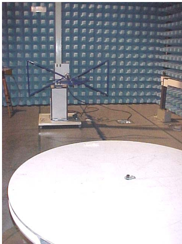
PHOTO N° 2 – SET-UP FOR EMISSION RADIATED TEST
