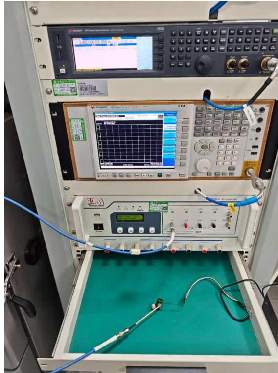
Antenna Terminal Test View
