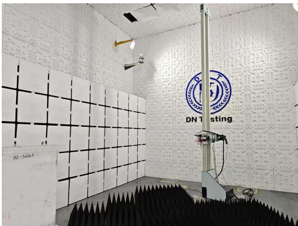
Radiated Emission Test View|(Above 1G)
