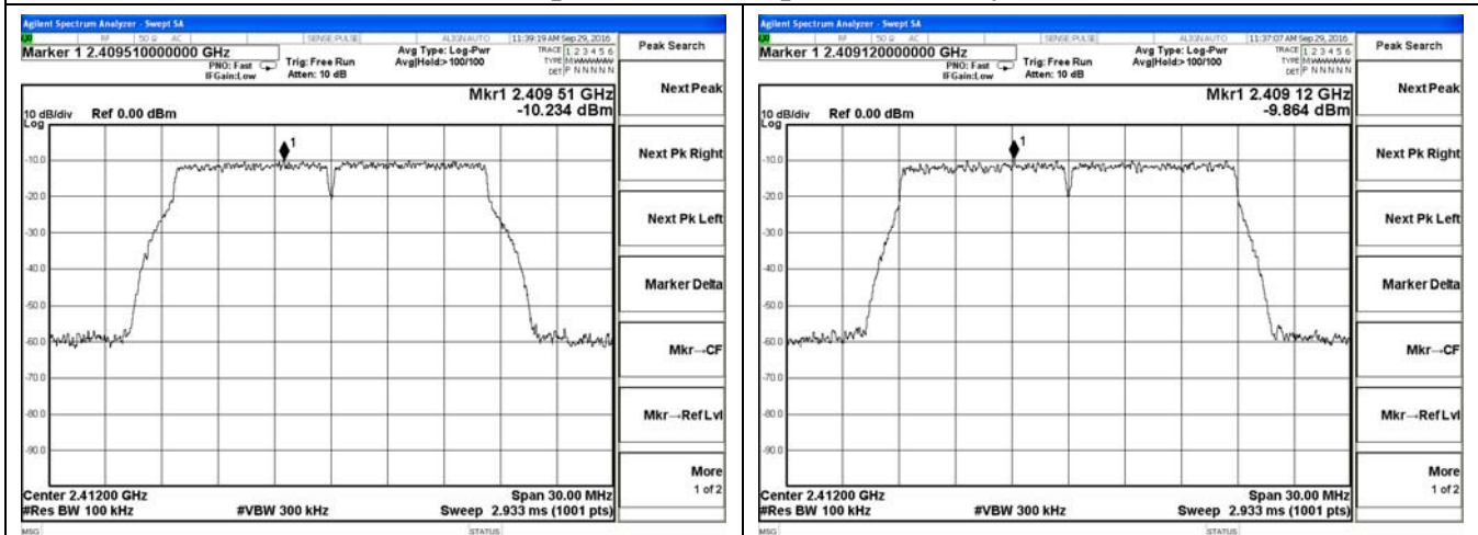
802.11g-Low Channel
