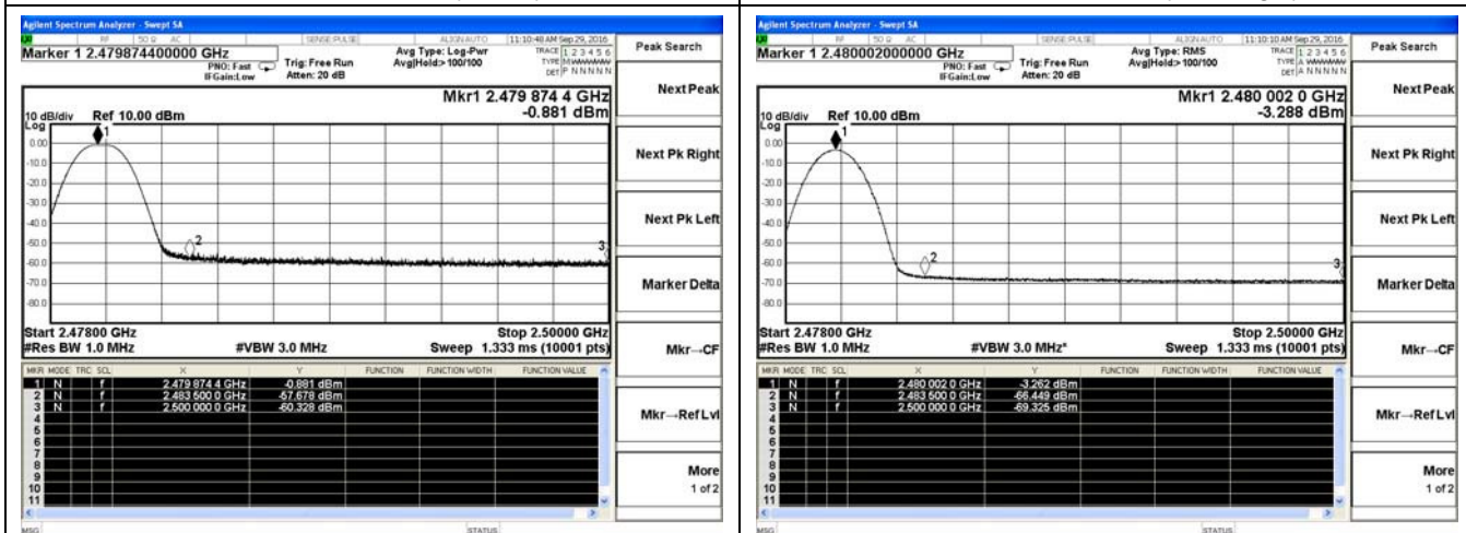
BLE-High channel(Peak)
