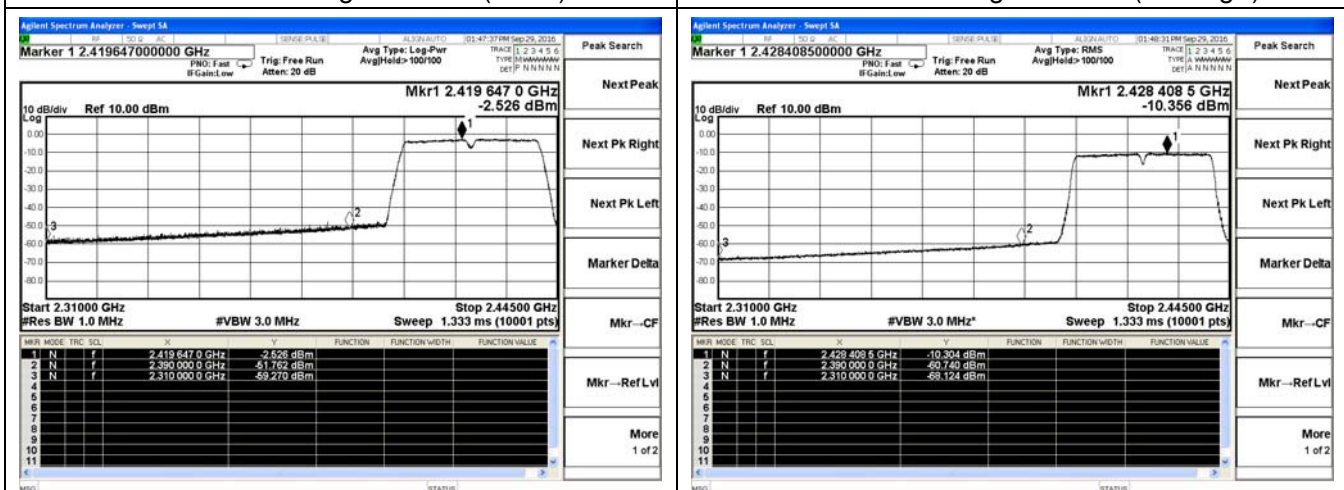
802.11n-HT40-Low channel(Peak)
