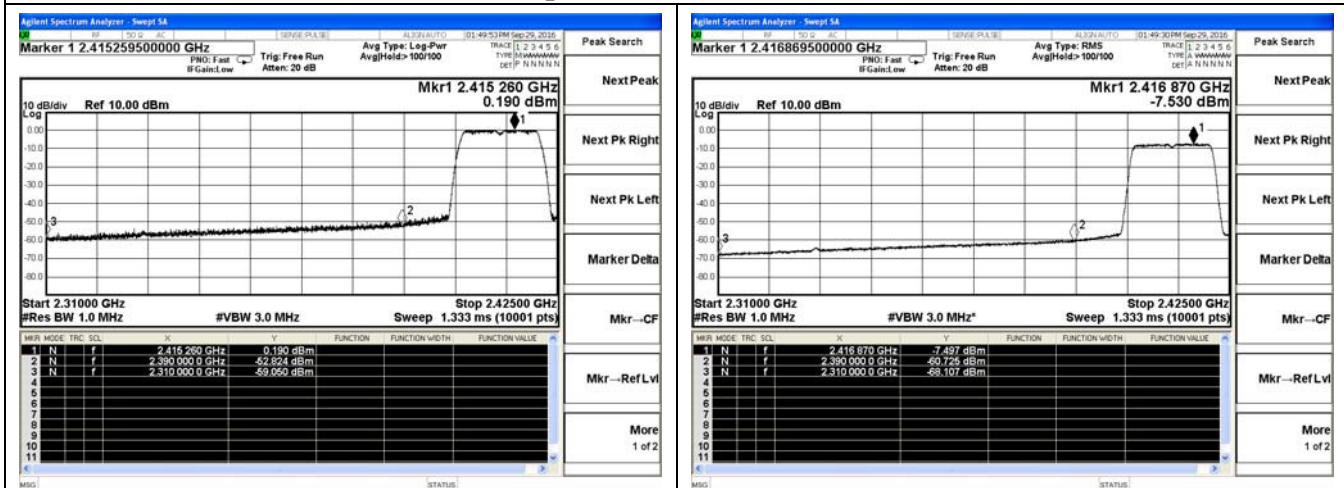
802.11n-HT20-Low channel(Peak)
