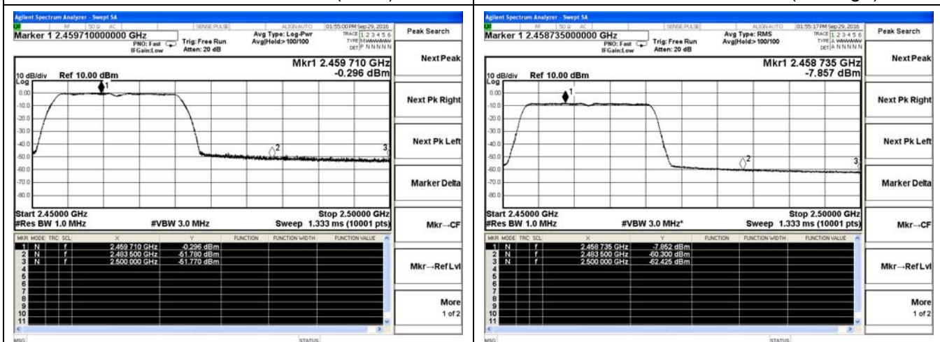
802.11n-HT20-High channel(Peak)
