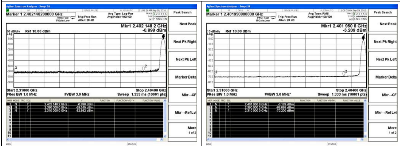
BLE-Low channel(Peak)
