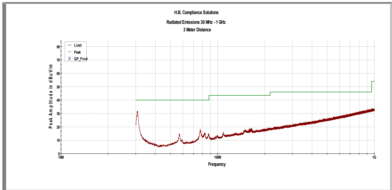
Plot 2 – Radiated Emissions – 30MHz to 1GHz – Charging
