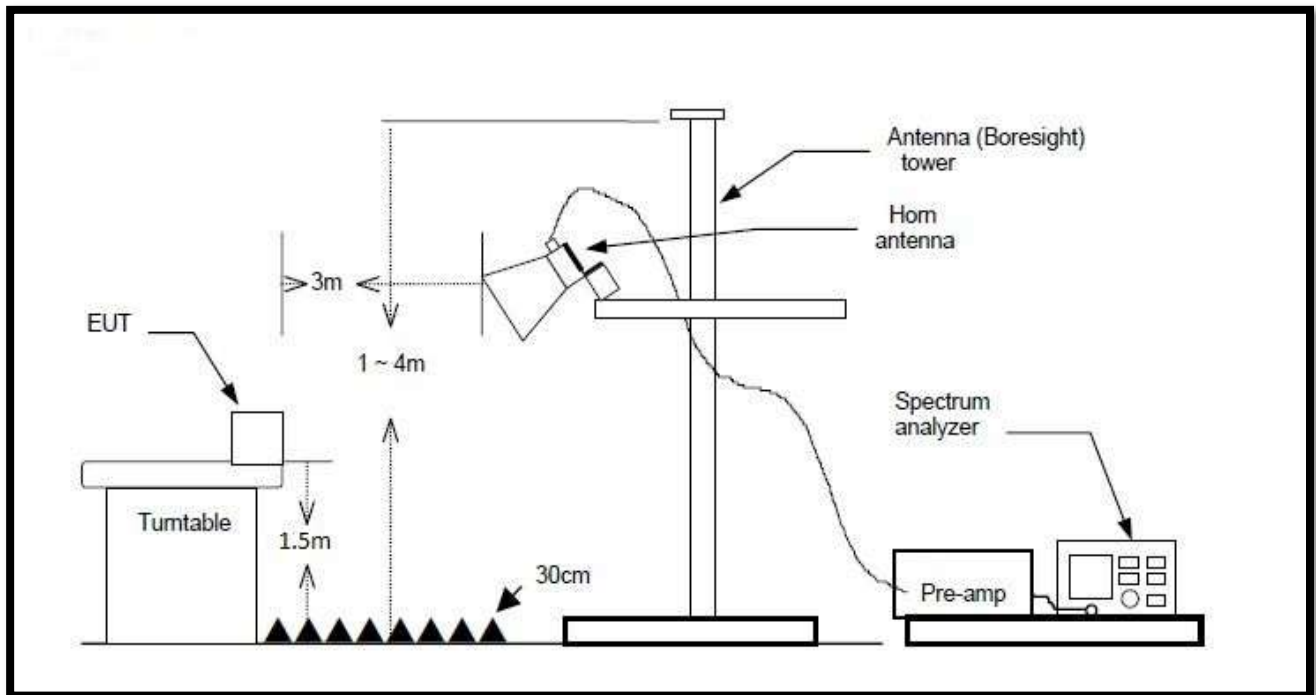
Figure 4. Radiated Emission Above 1GHz Test Setup
