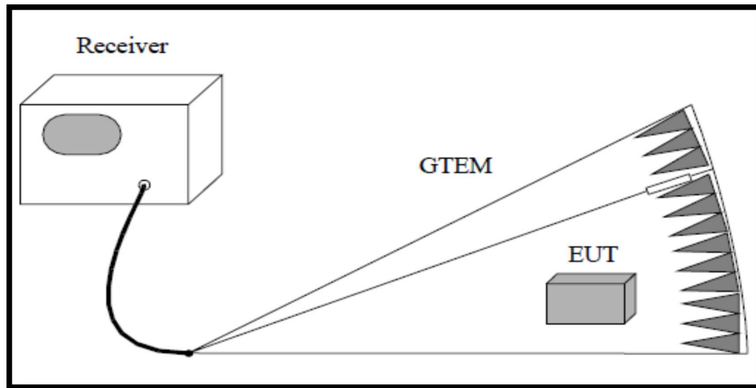
Figure 1. Radiated Emissions Test Setup (30MHz – 1GHz)
