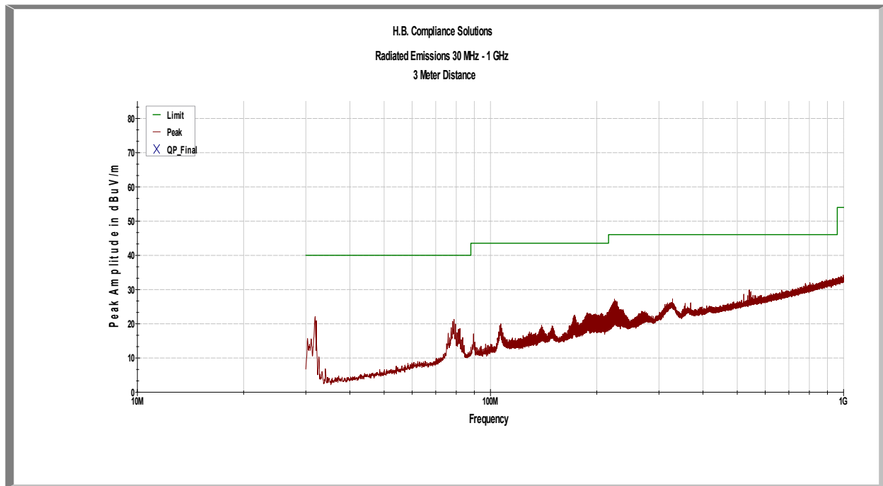
Plot 1 – Radiated Emissions – 30MHz to 1GHz – Idle Mode
