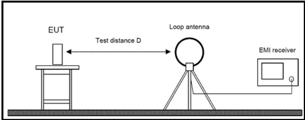
Figure 3. Radiated Emissions Test Setup (9kHz - 30MHz)
