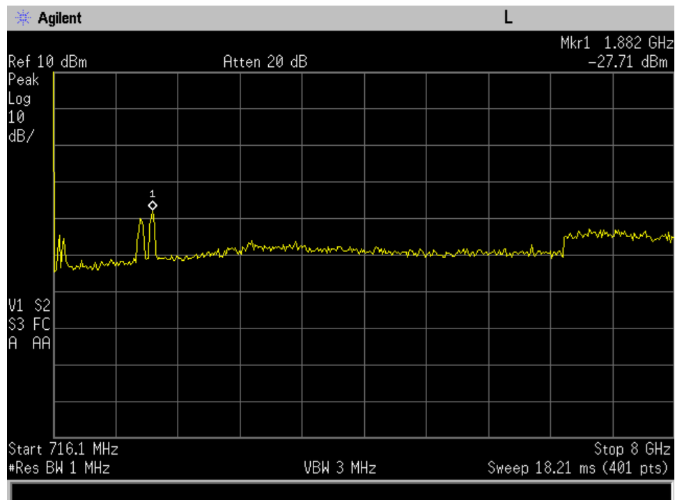
Uplink_698 - 716 MHz_plot 2
