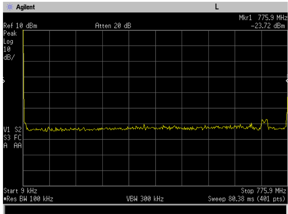
Uplink_776 - 787 MHz_plot 1
