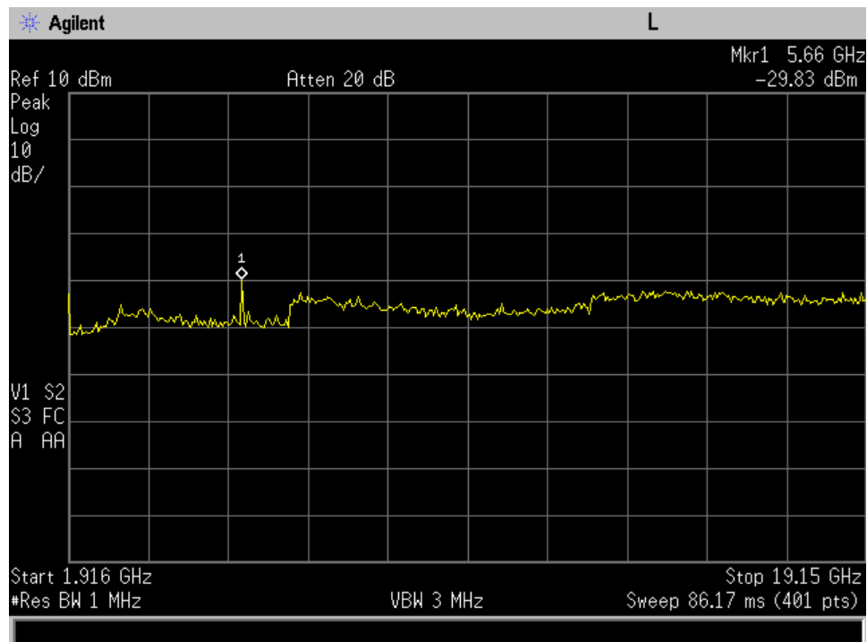
Uplink_1850 - 1910 MHz_plot 2
