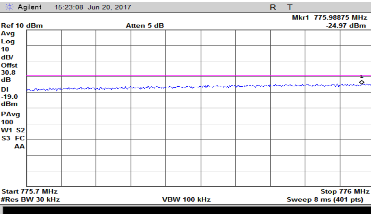
Plot 32 – 776-787MHz Band – CDMA Uplink Lower Band Edge
