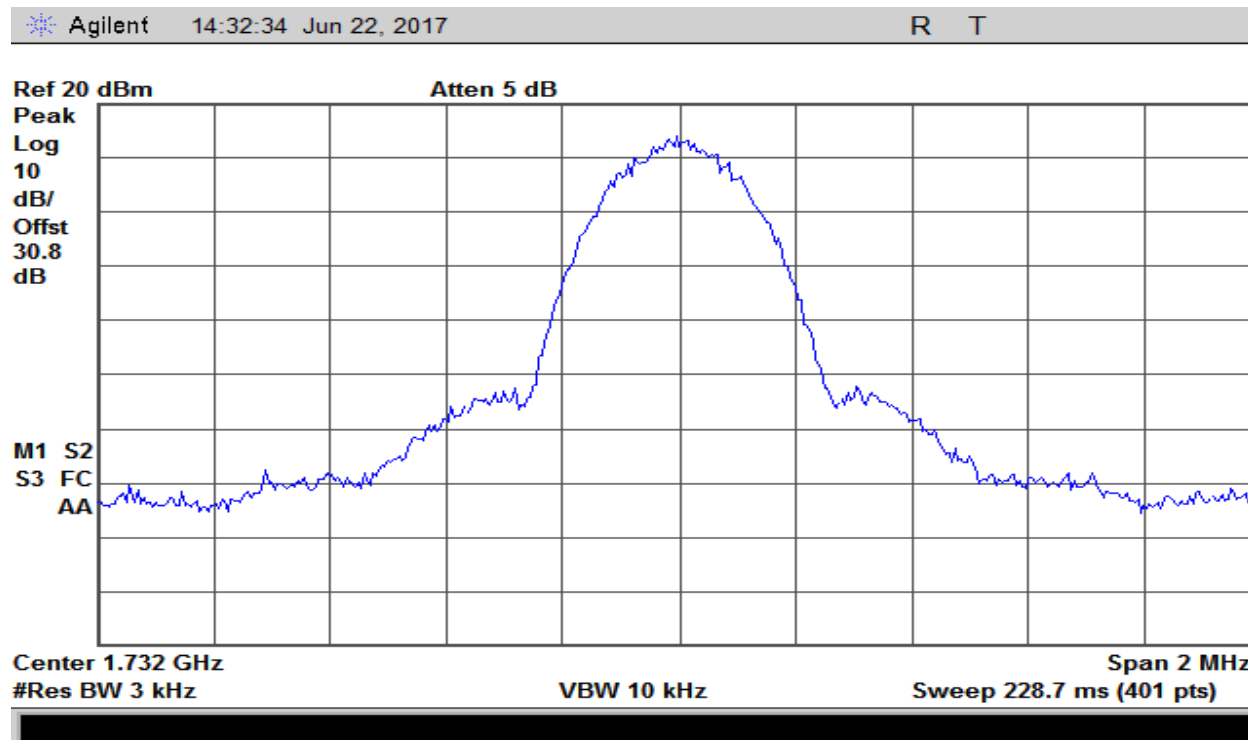
Plot 138 – 1710-1755MHz Band – Uplink Output – GSM
