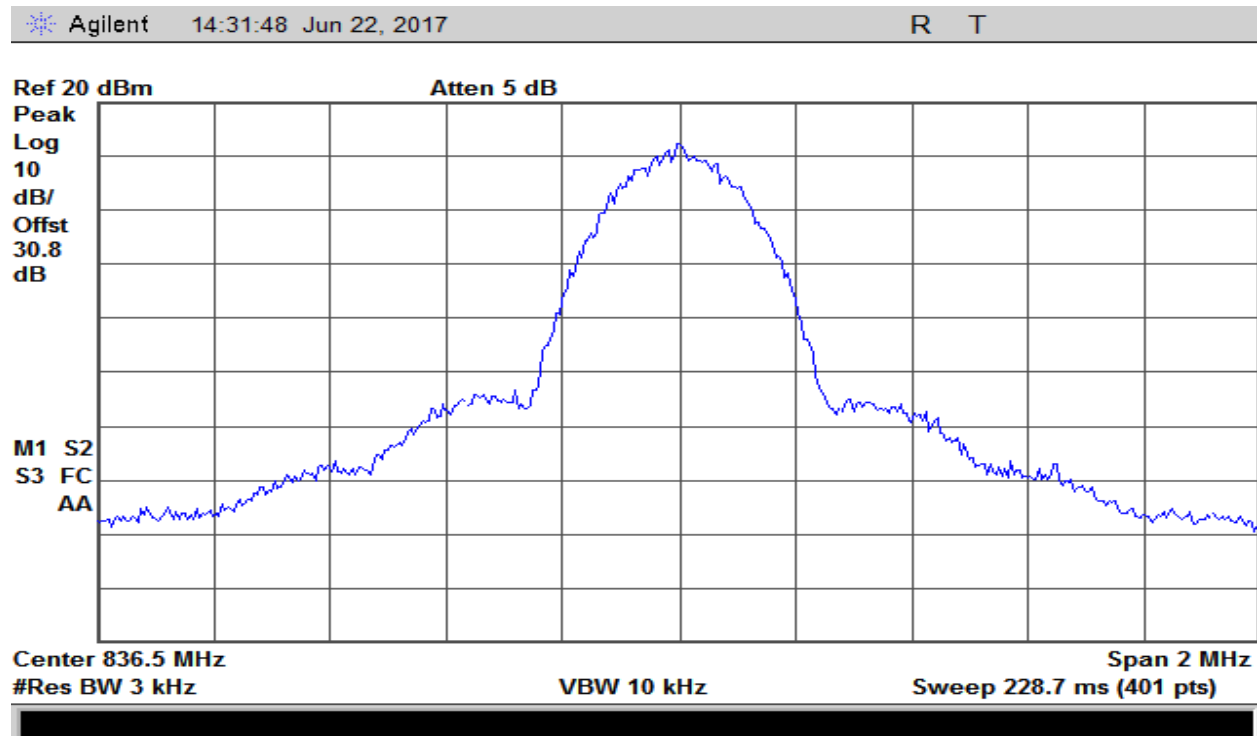
Plot 136 – 824-849MHz Band – Uplink Output – GSM
