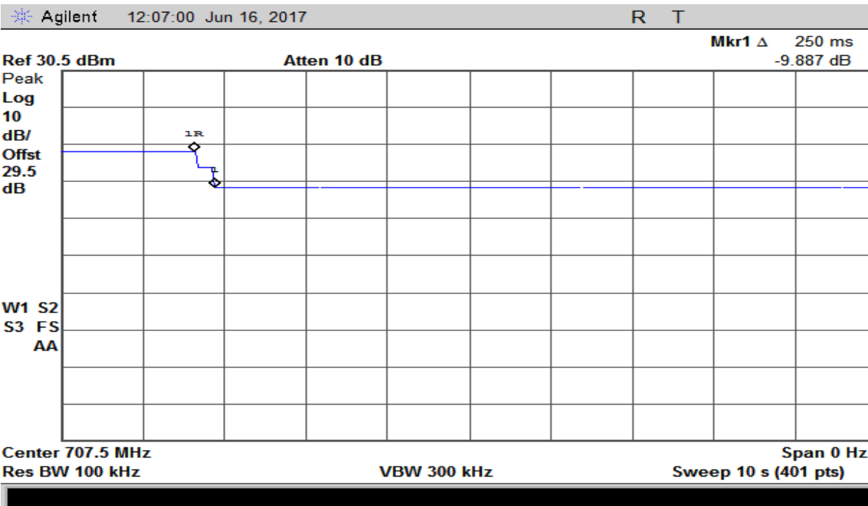
Plot 126 – 698-716MHz Band – Uplink Gain Timing
