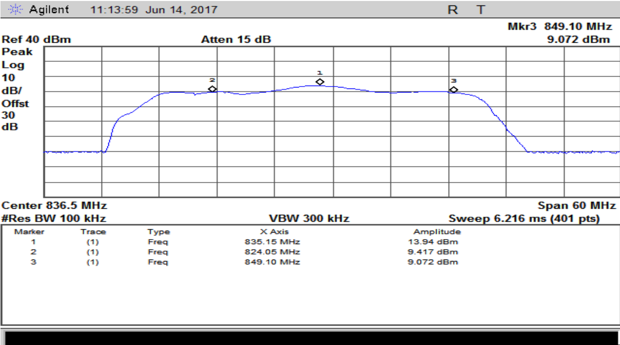
Plot 3 – 824-849MHz Band – Uplink
