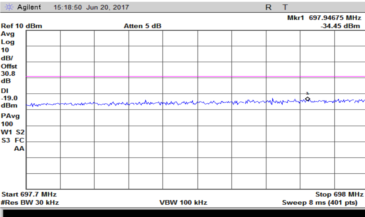
Plot 30 – 698-716MHz Band – CDMA Uplink Lower Band Edge
