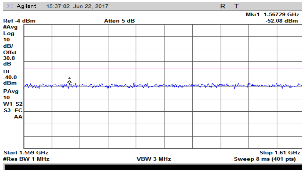
Plot 116 -27.53f - Uplink Wideband
