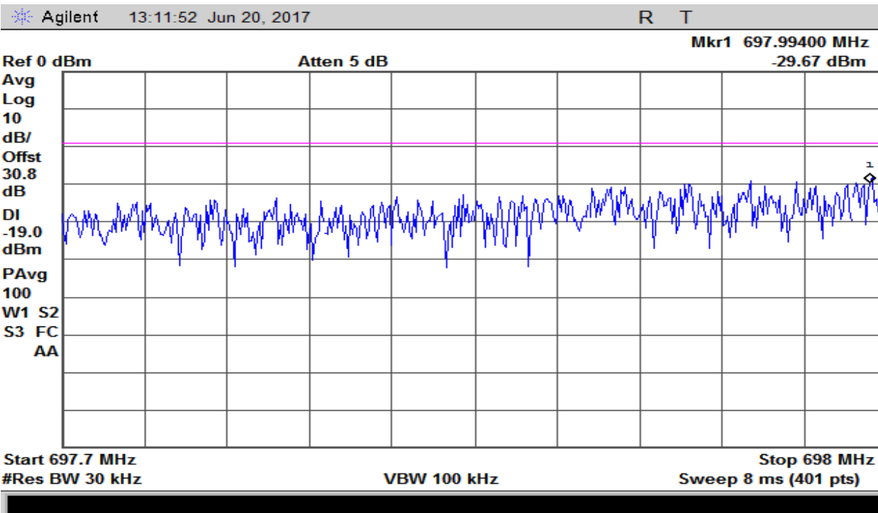
Plot 21 – 698-716MHz Band – GSM Uplink Lower Band Edge
