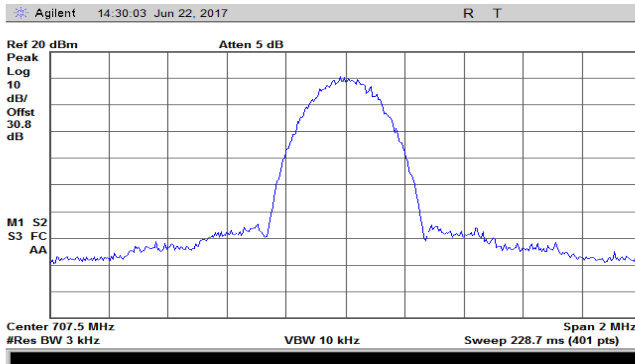
Plot 132 – 698-716MHz Band – Uplink Output – GSM
