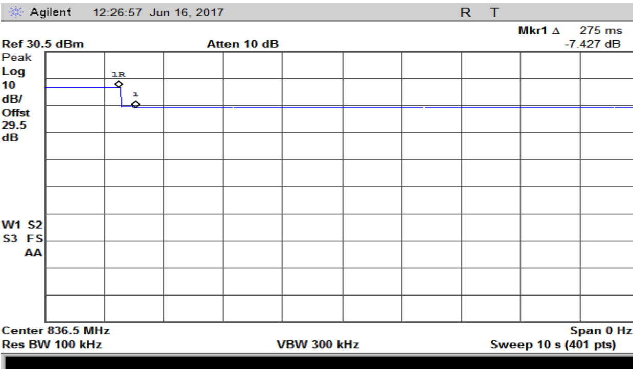
Plot 128 – 824-849MHz Band – Uplink Gain Timing
