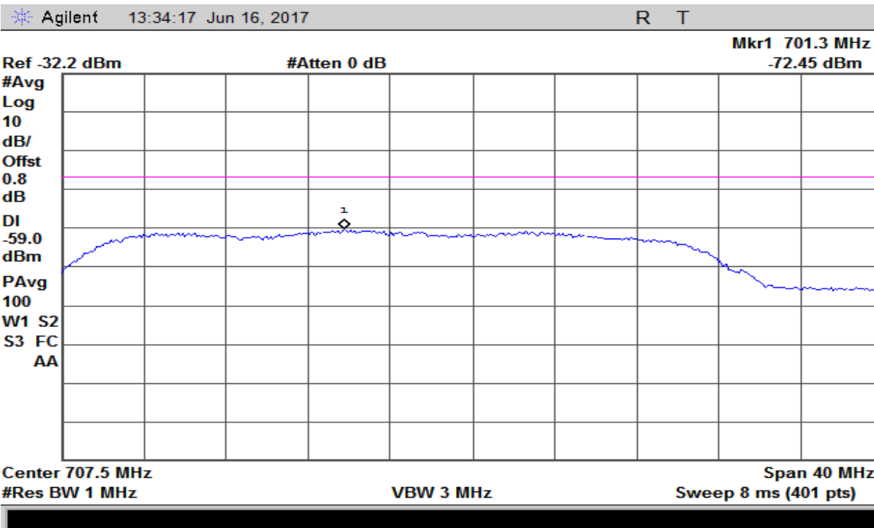
Plot 121 – 698-716MHz Band – Maximum Uplink Noise
