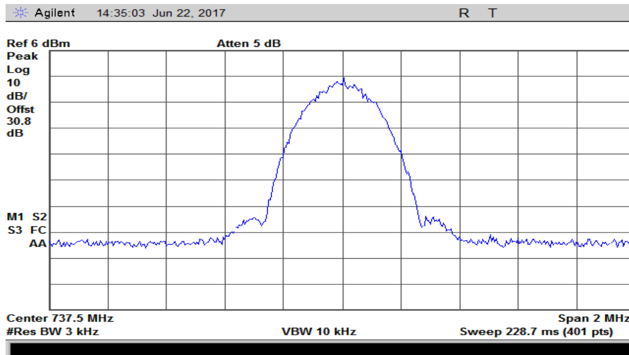
Plot 142 – 728-746MHz Band – Downlink Output – GSM
