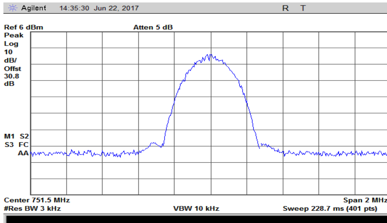
Plot 144 – 746-757MHz Band – Downlink Output – GSM
