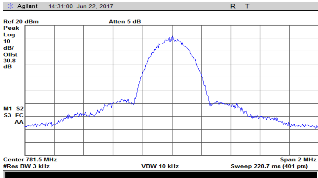
Plot 134 – 776-787MHz Band – Uplink Output – GSM
