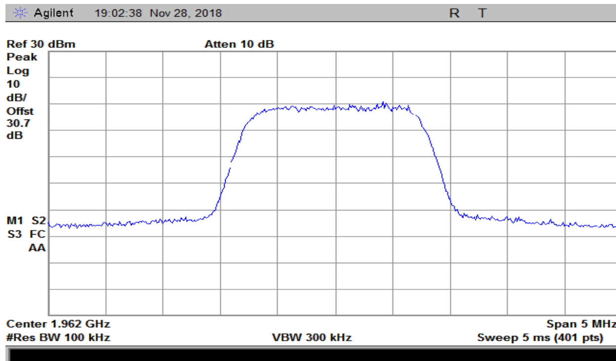
Plot 178 – 1930-1995MHz Band – Downlink Output – CDMA
