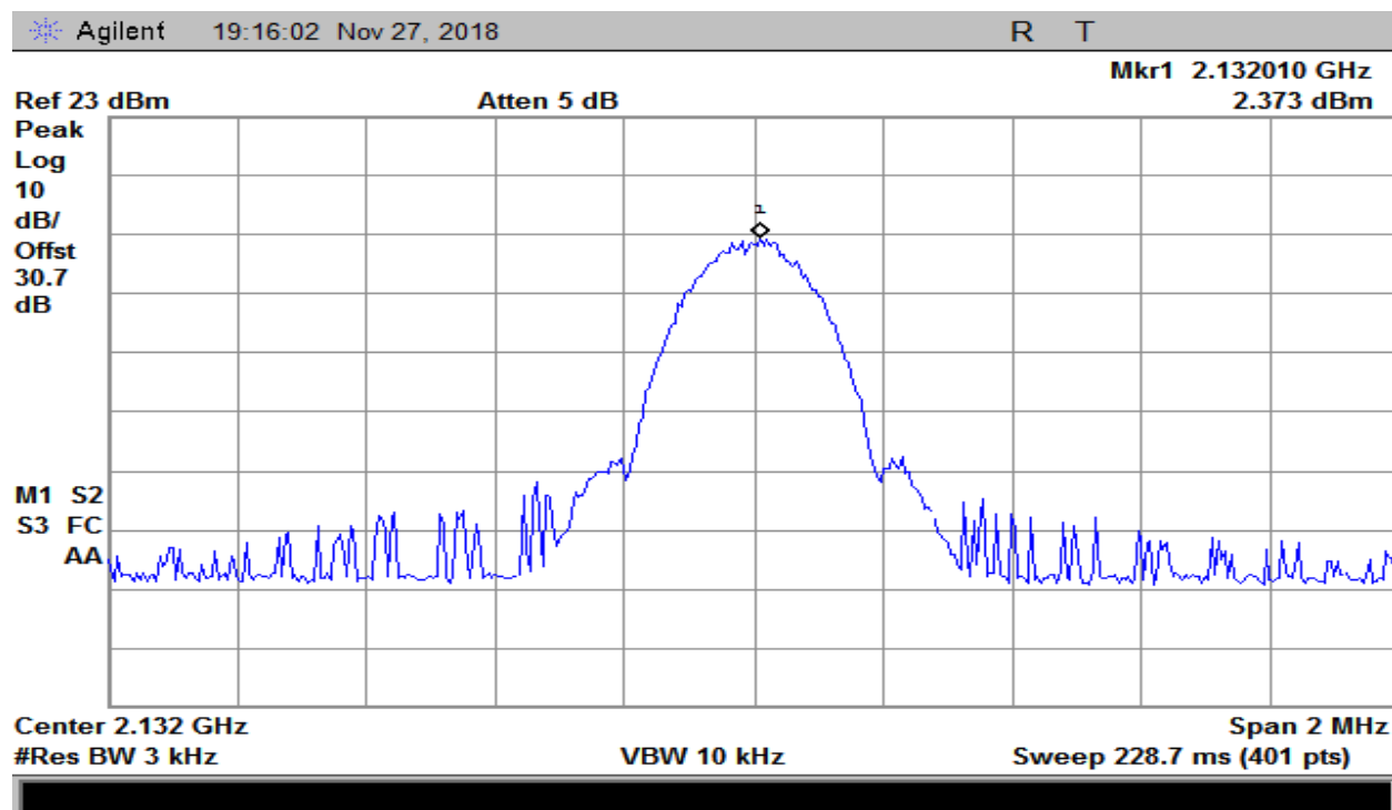
Plot 160 – 2110-2155MHz Band – Downlink Output – GSM
