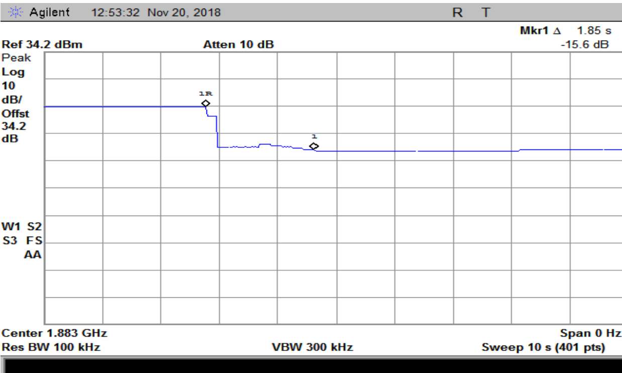
Plot 140 – 1850-1915MHz Band – Uplink Gain Timing
