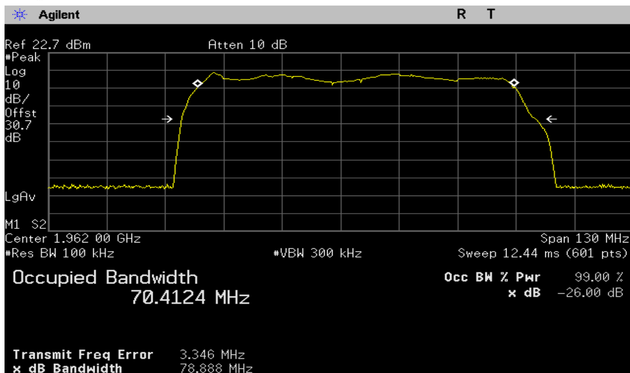
Plot 209 – 1930-1995MHz Band – Downlink – 99% BW for ISED (Canada)
