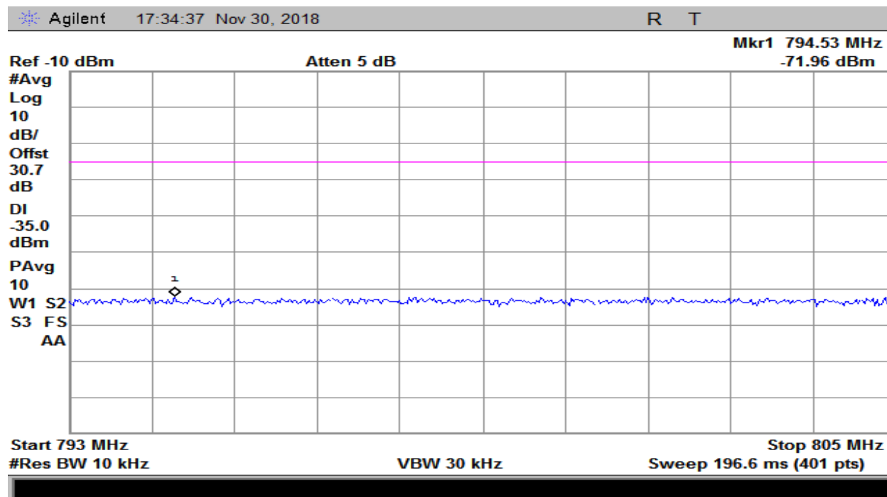
Plot 121 -27.53c4 – Downlink
