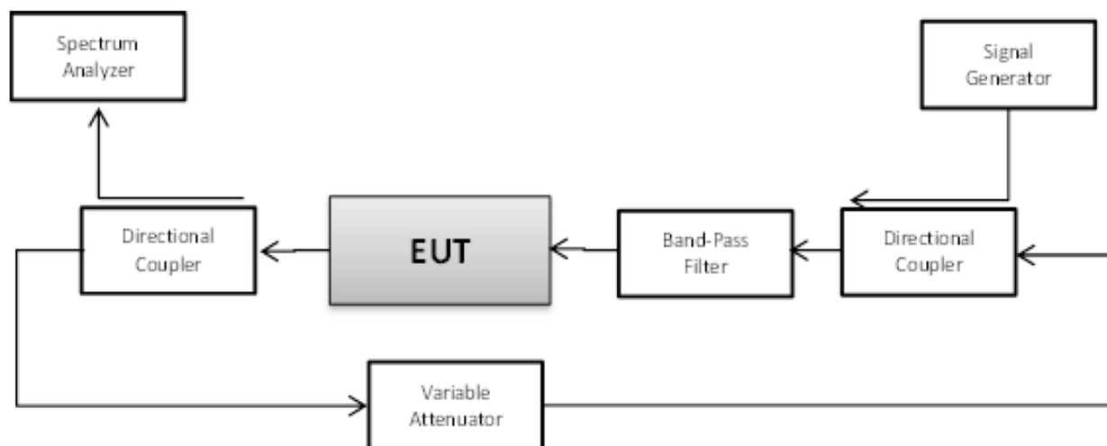
Figure 5 – Oscillation mitigation/shutdown
