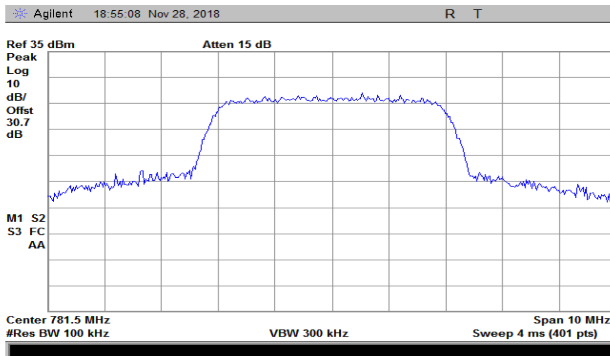
Plot 184 – 776-787MHz Band – Uplink Output – LTE
