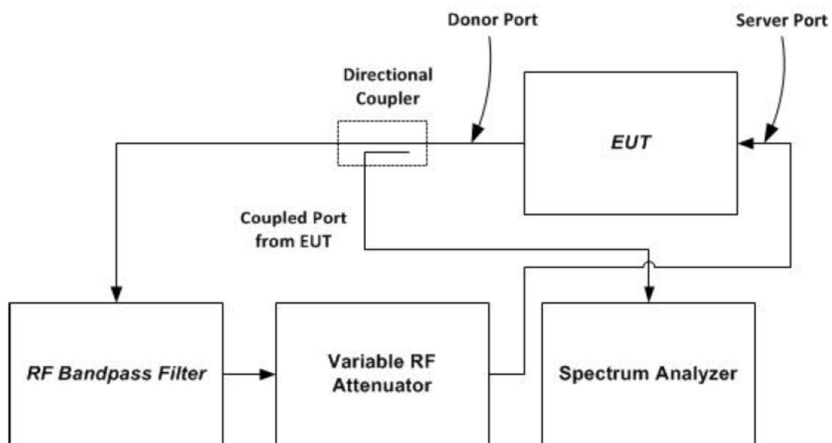
Figure 4 – Oscillation detection
