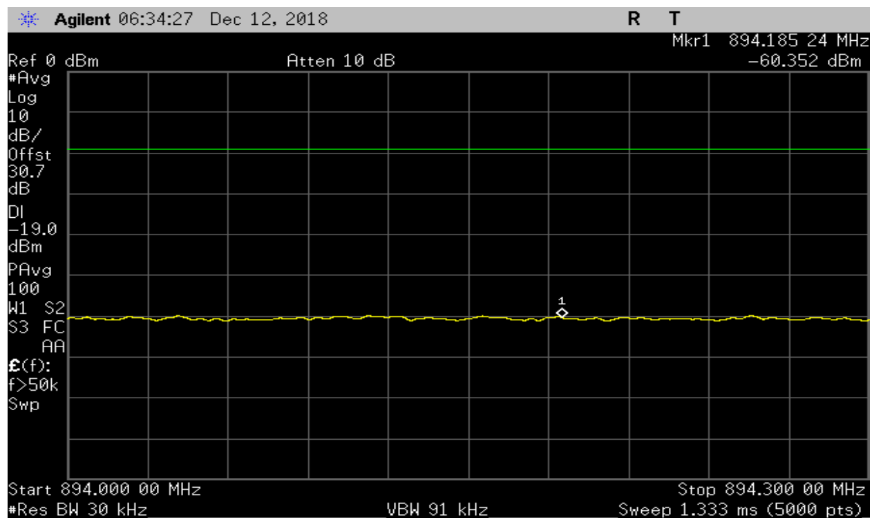
Plot 75 – 869-894MHz Band – LTE Downlink Upper Band Edge
