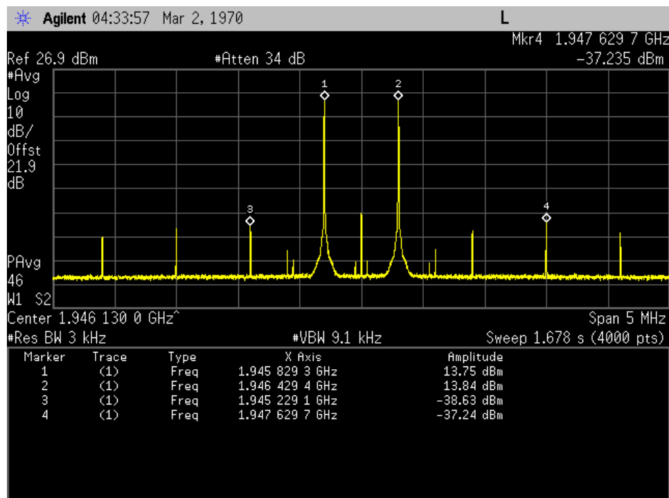
Intermodulation_Downlink_1930-1995 MHz_Server Port to D1
