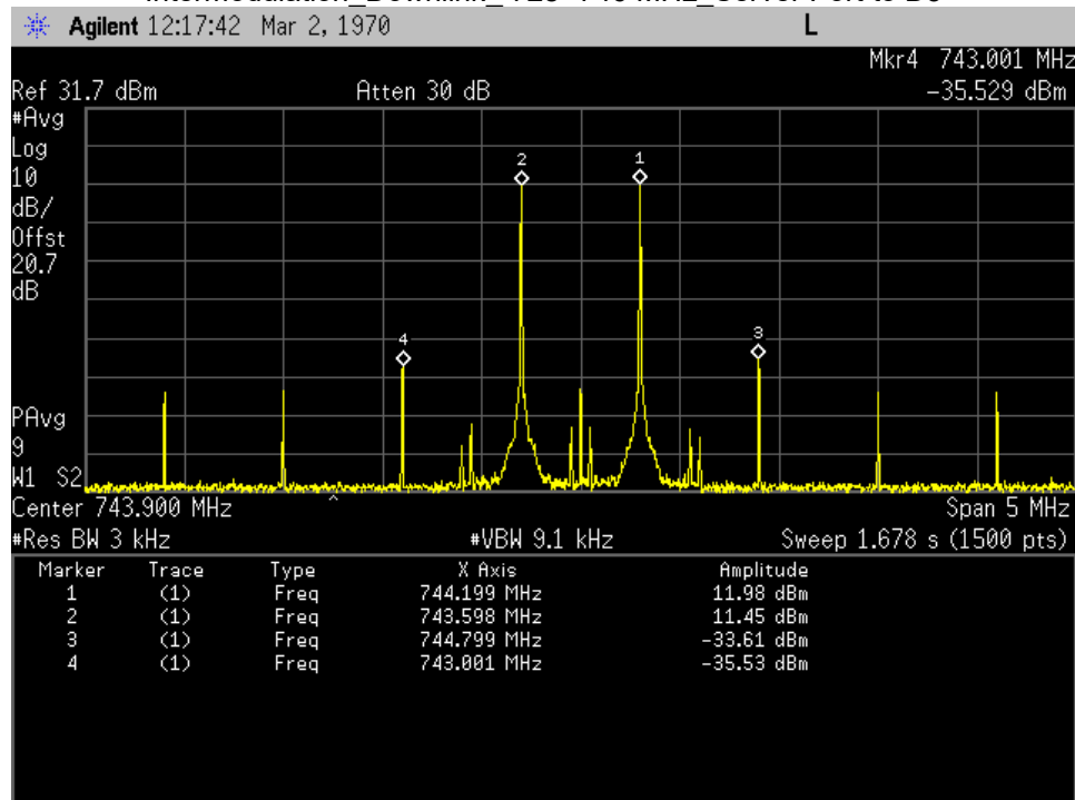
Intermodulation_Downlink_728-746 MHz_Server Port to D3
