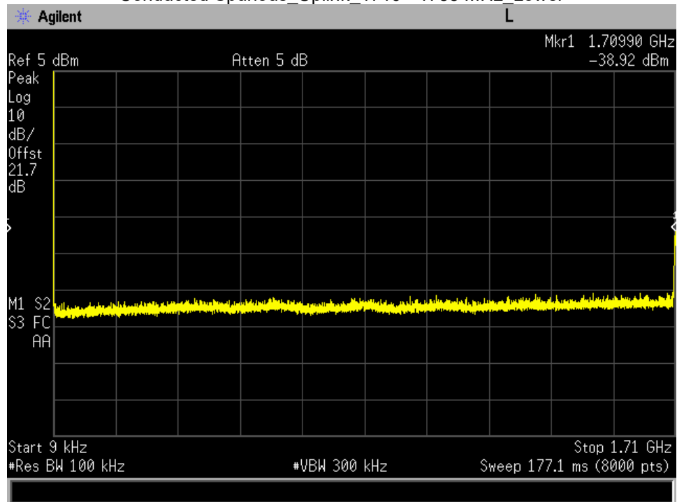
Conducted Spurious_Uplink_1710 - 1755 MHz_Lower
