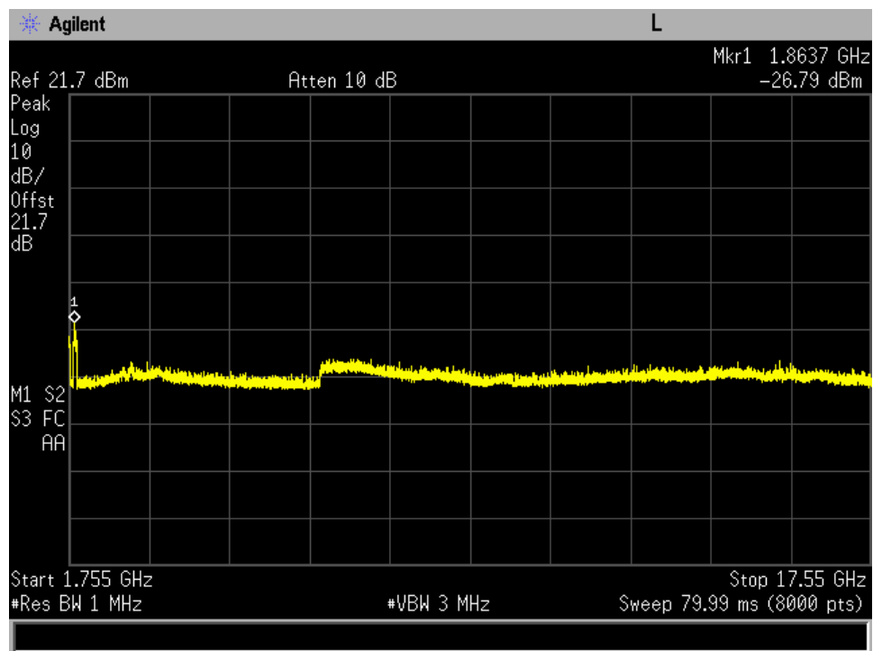
Conducted Spurious_Uplink_1710 - 1755 MHz_Upper
