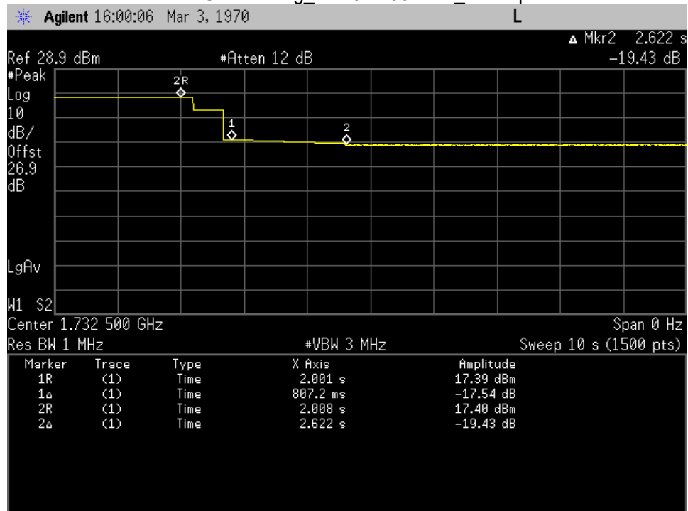
Variable Gain Timing_ 1710-1755 MHz_donor port 1
