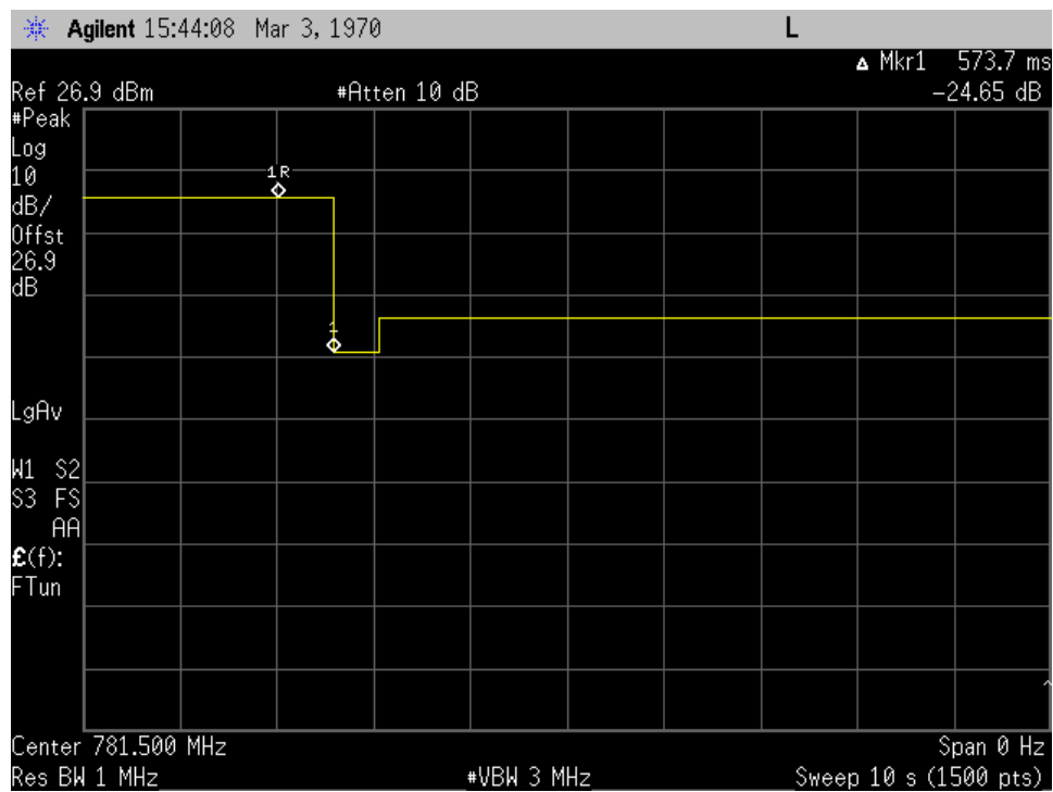
Variable Gain Timing_ 776-787 MHz_donor port 1
