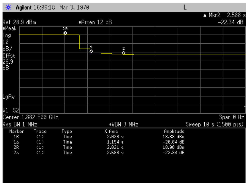
Variable Gain Timing_ 1850-1915 MHz_donor port 1
