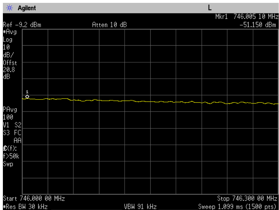
OOBE_DL_CDMA_728 - 746 MHz_Upper_Common Donor Port 1
