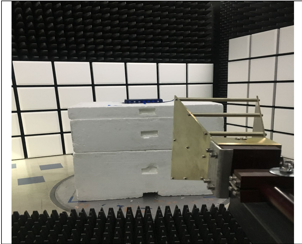
RF Radiated 1-18 GHz
