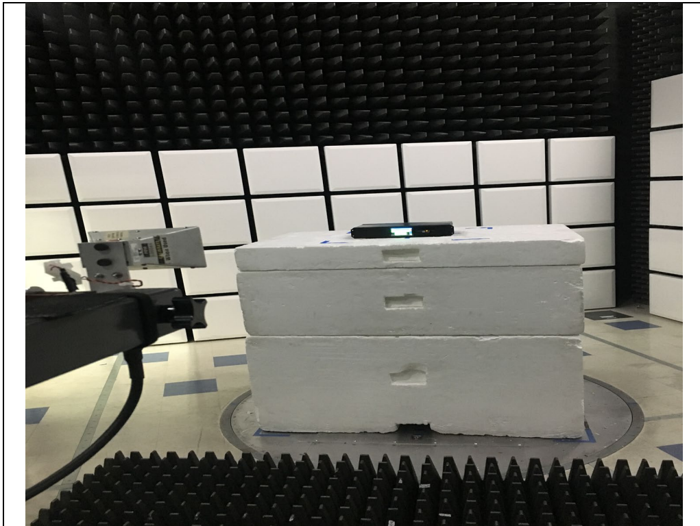
RF Radiated 18-26 GHz
