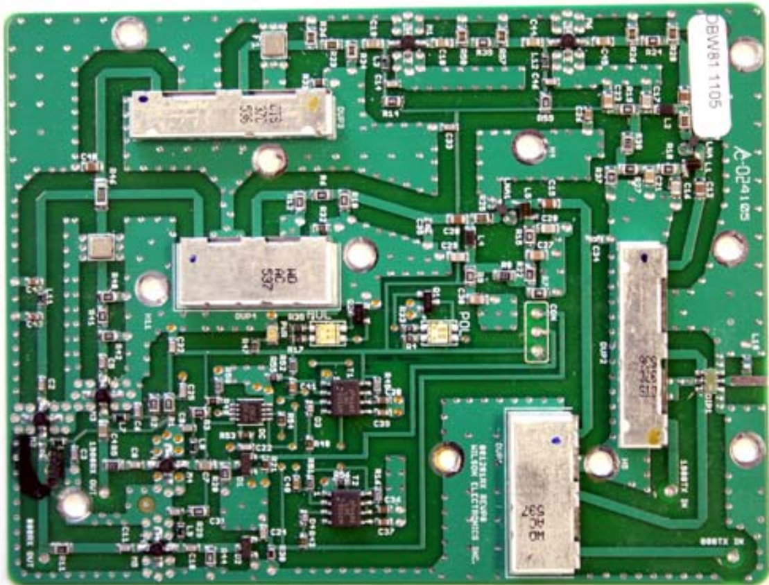
Top Board
