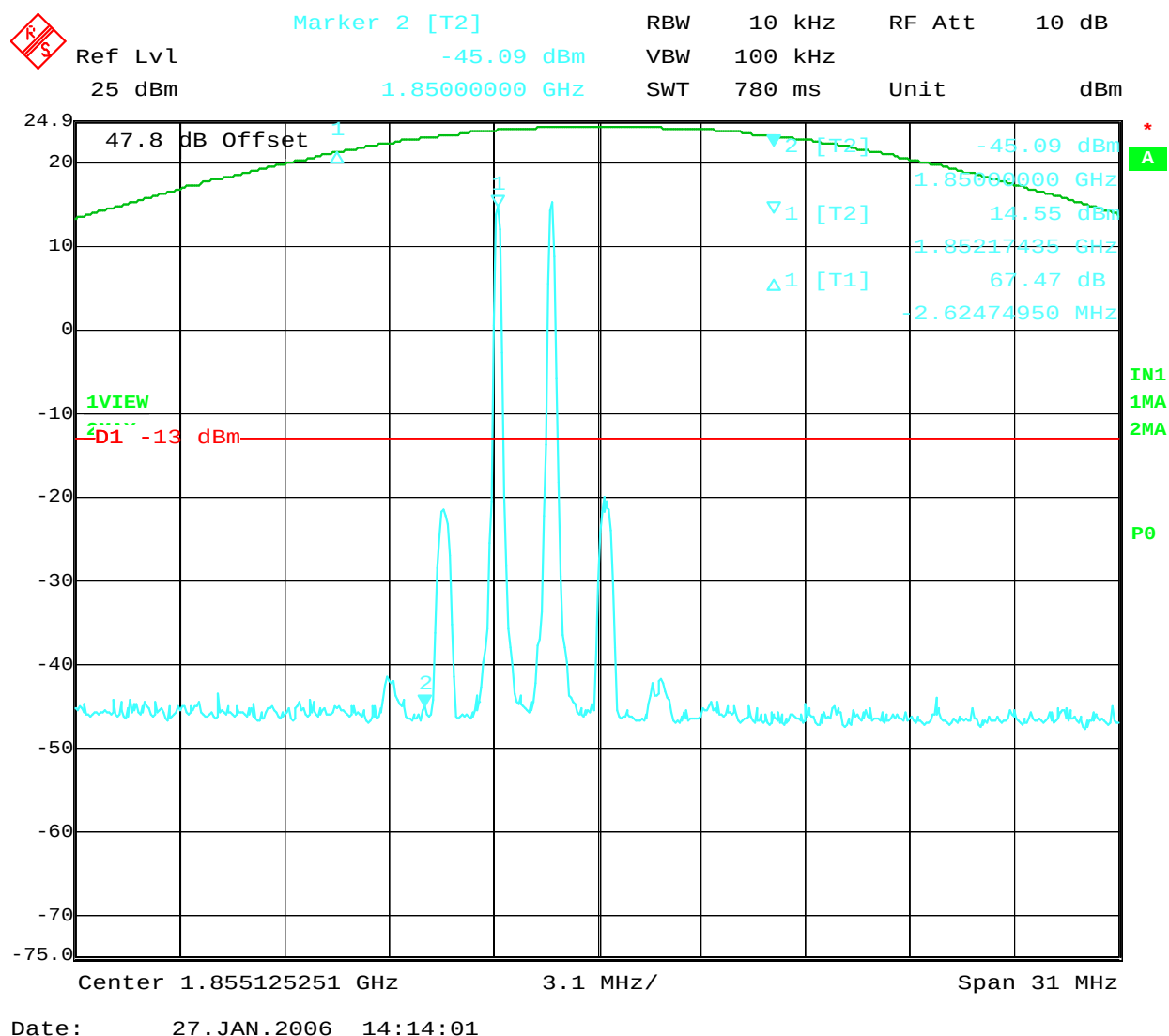
Figure 16: Intermodulation 3 tones sprurious emissions (zoom in) GSM up link.
