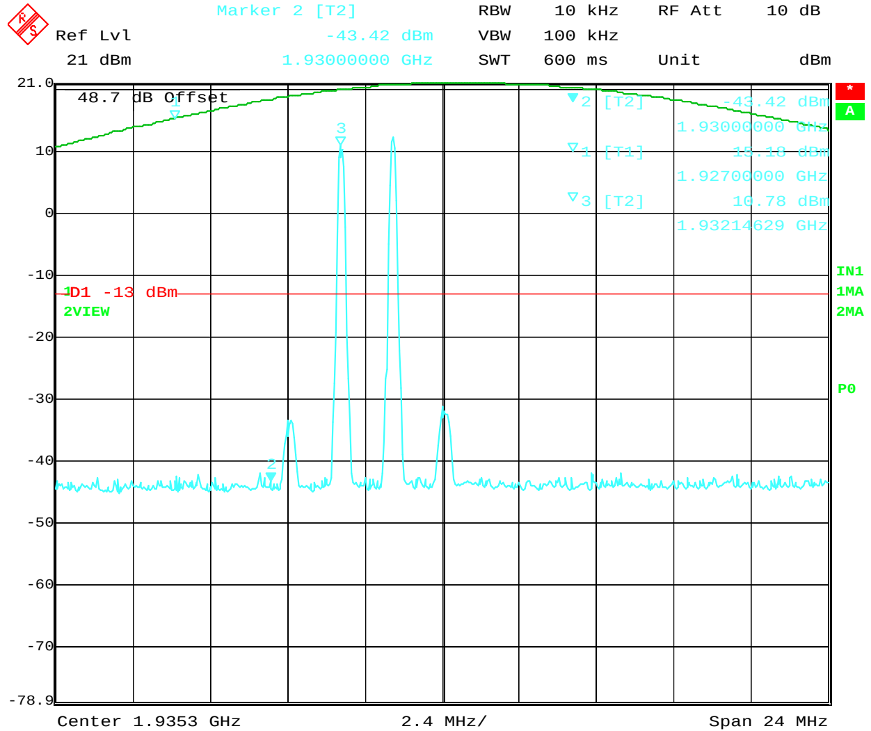
Figure 18: Intermodulation 3 tones sprurious emissions (zoom in) GSM down link.
