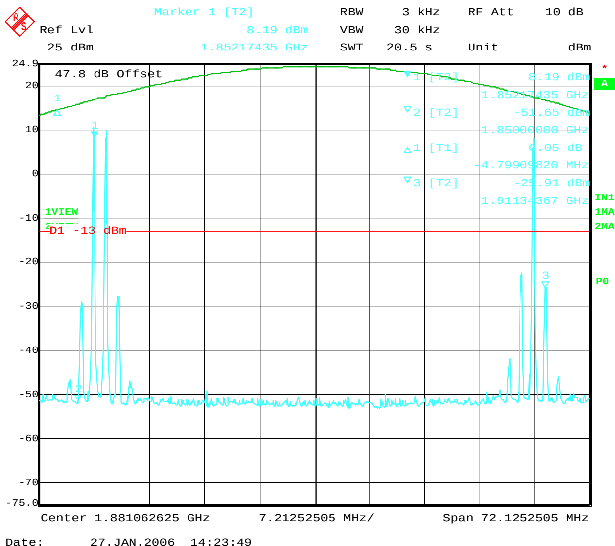
Figure 15: Intermodulation 3 tones sprurious emissions GSM up link.
