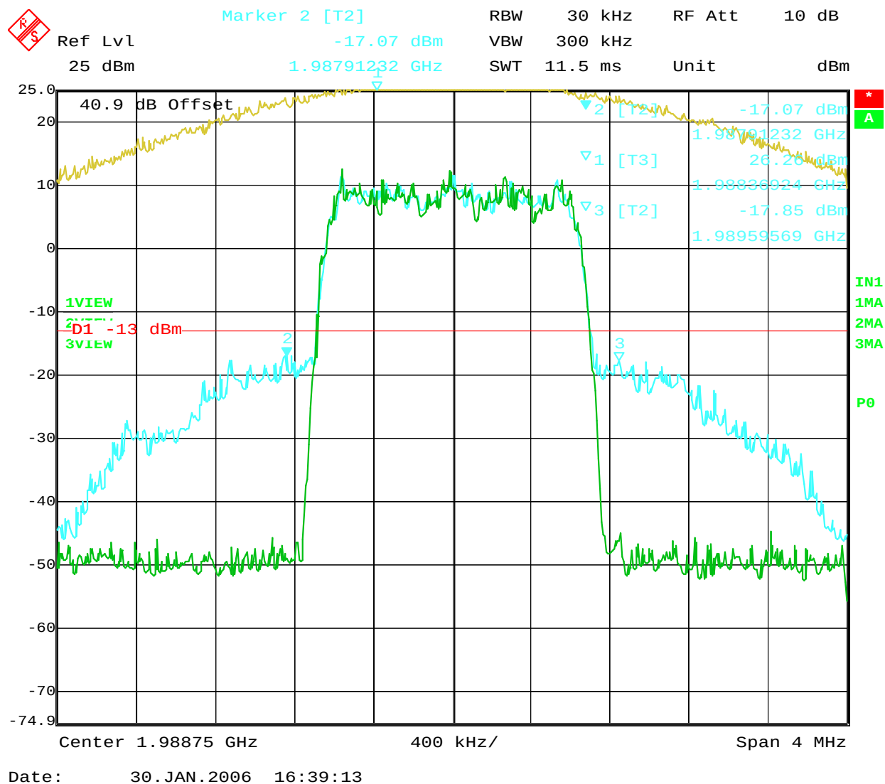
Figure 4: CDMA modulation - In vs. Out 1988.75MHz
