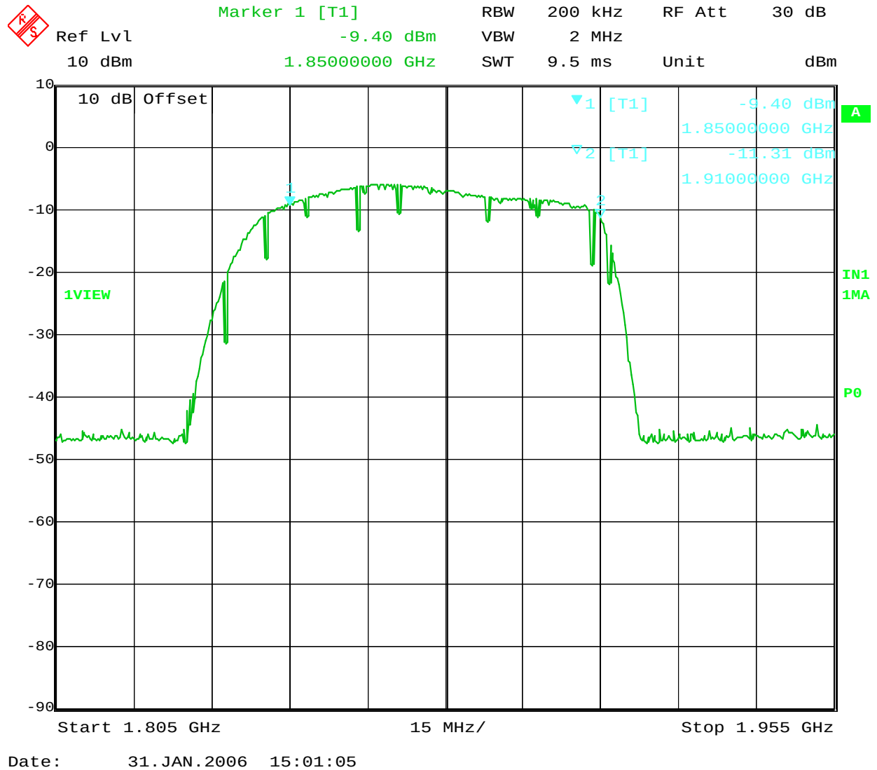
Figure 19. Filer frequency response 1850MHz band
