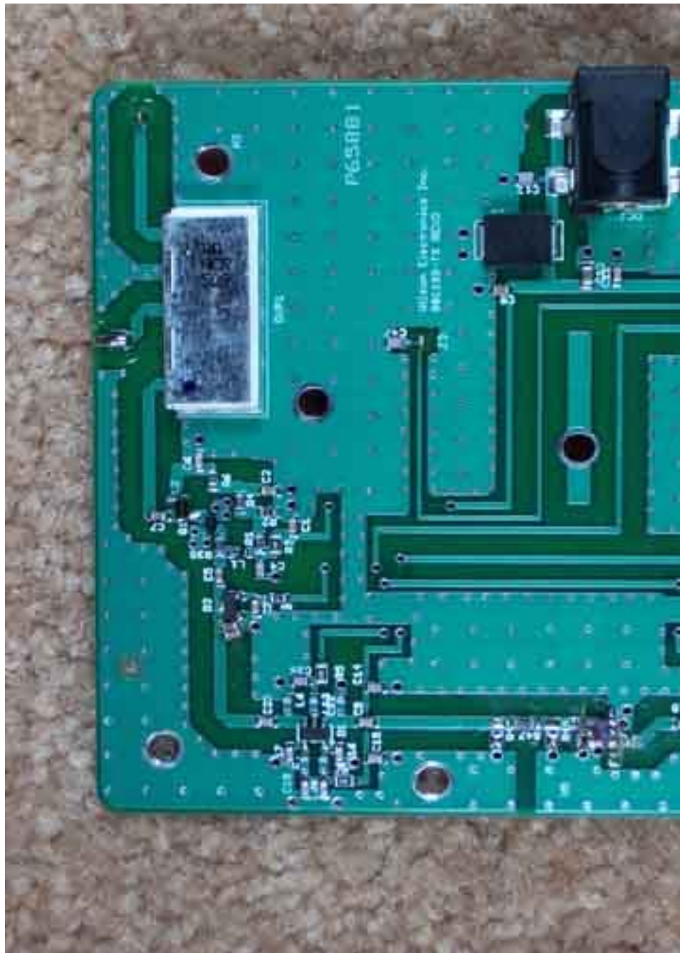
P65881 PCB Top Close-up 1
