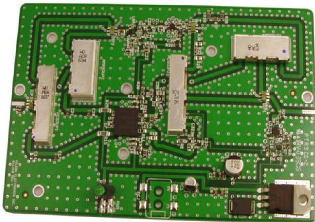
Board Top
