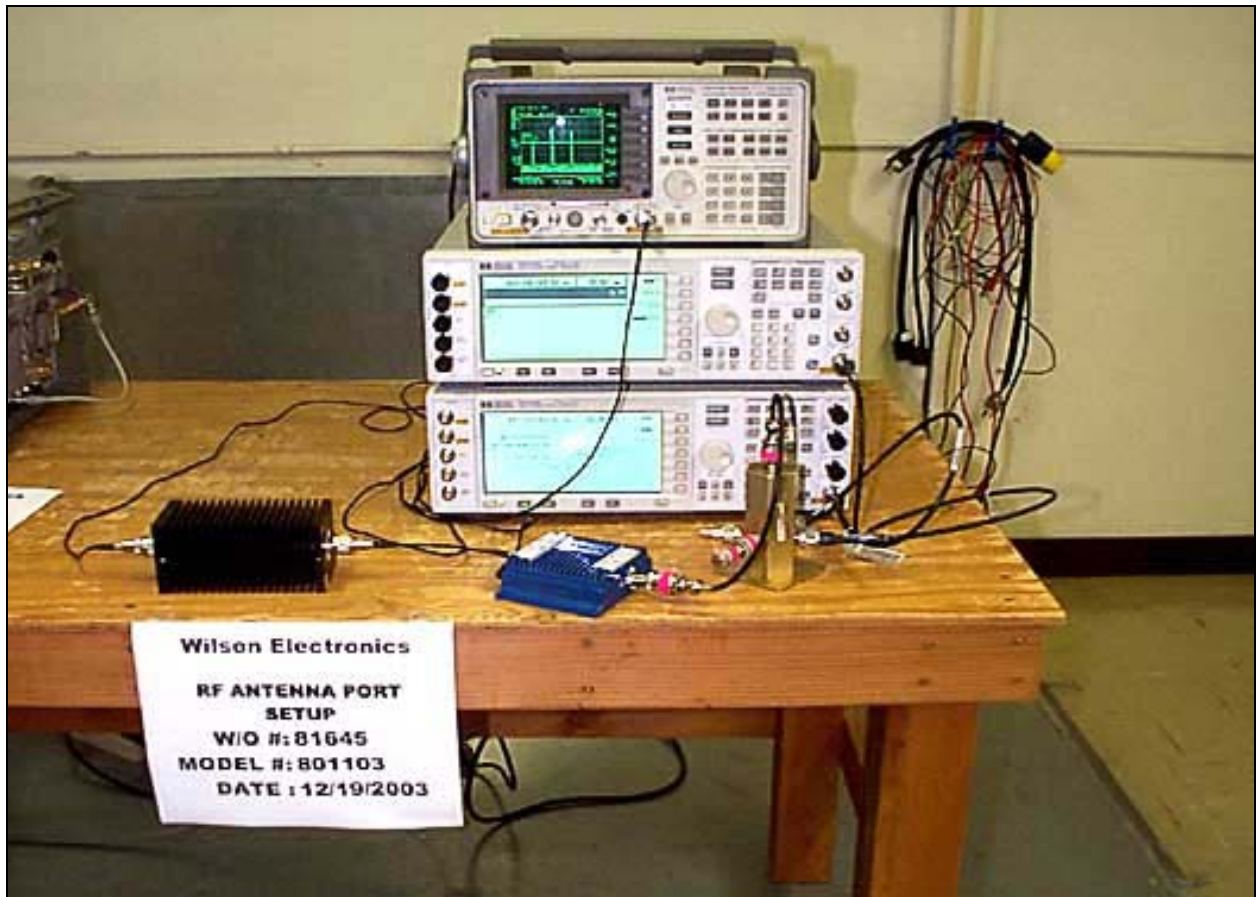
PHOTOGRAPH SHOWING DIRECT CONNECT
