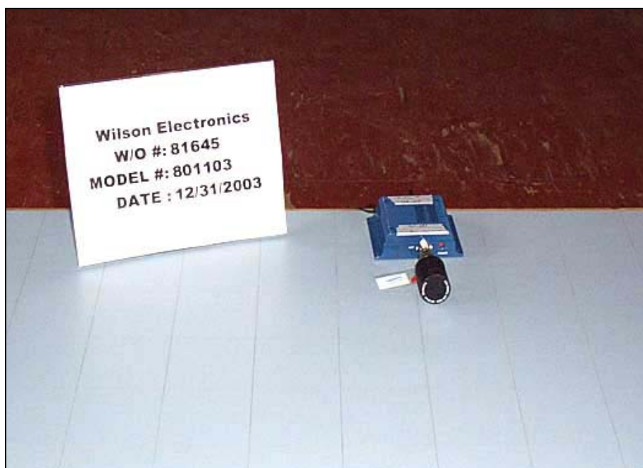
Radiated Emissions - Front View
