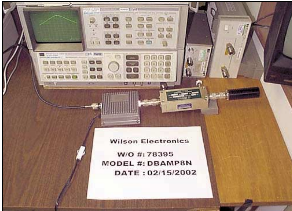
Antenna Direct Connect
