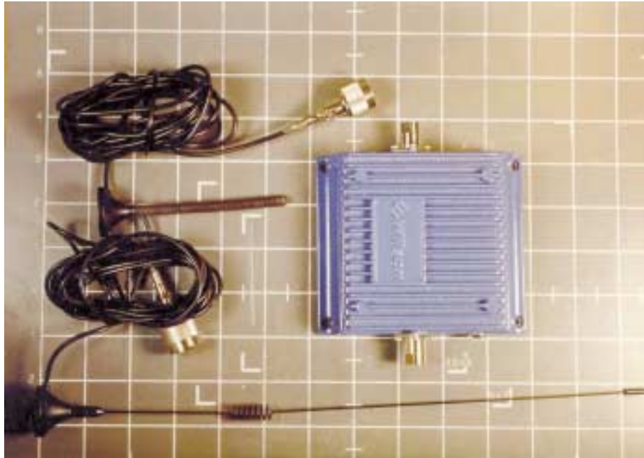
Overall with Antenna and EUT
