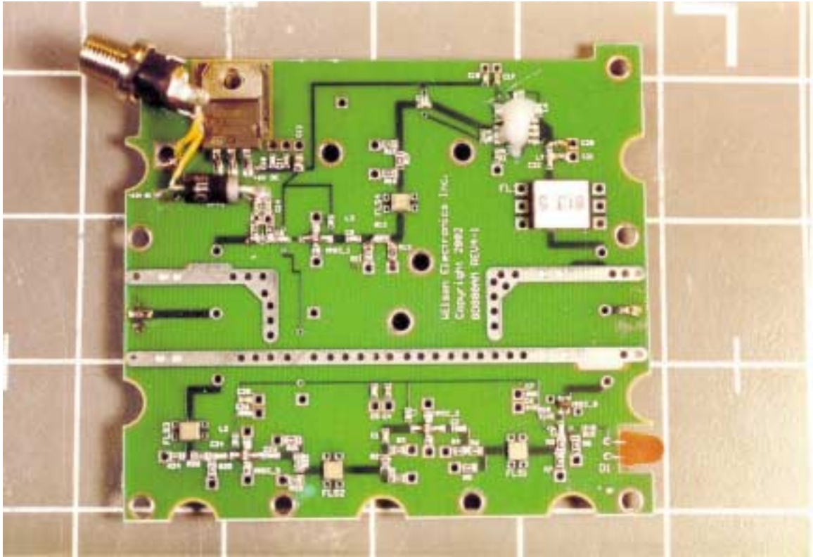
Top of PCB
