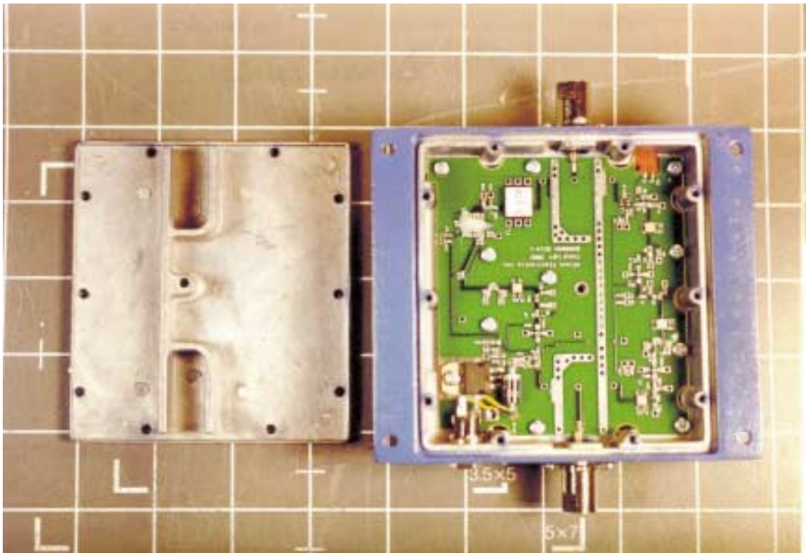
EUT with cover removed
