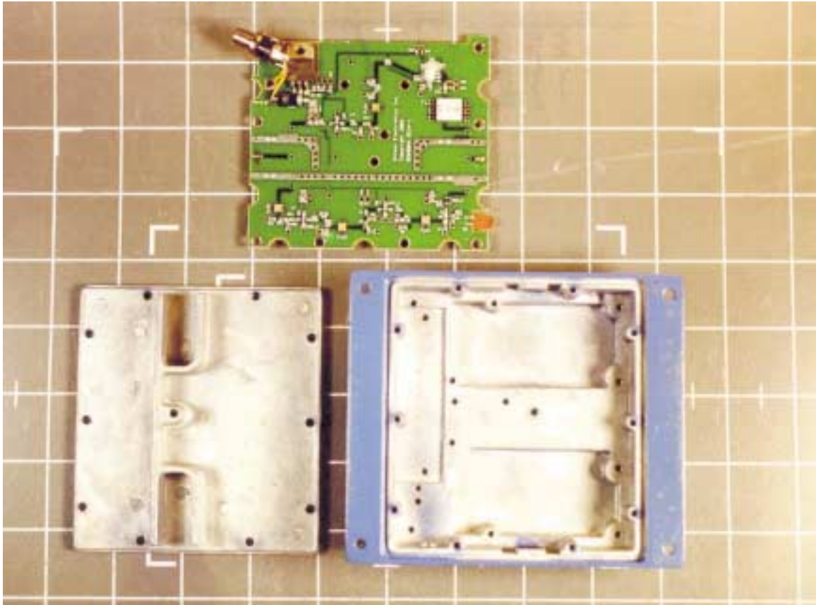
Overall with PCB removed
