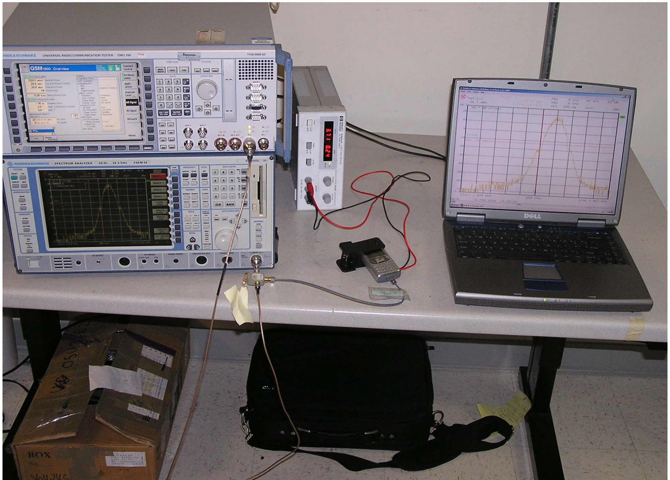
Test Setup RF conducted
