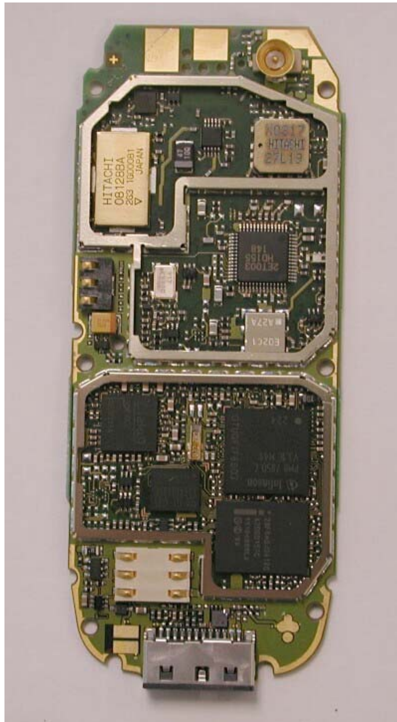
A56 Board without shielding lids, side 2
