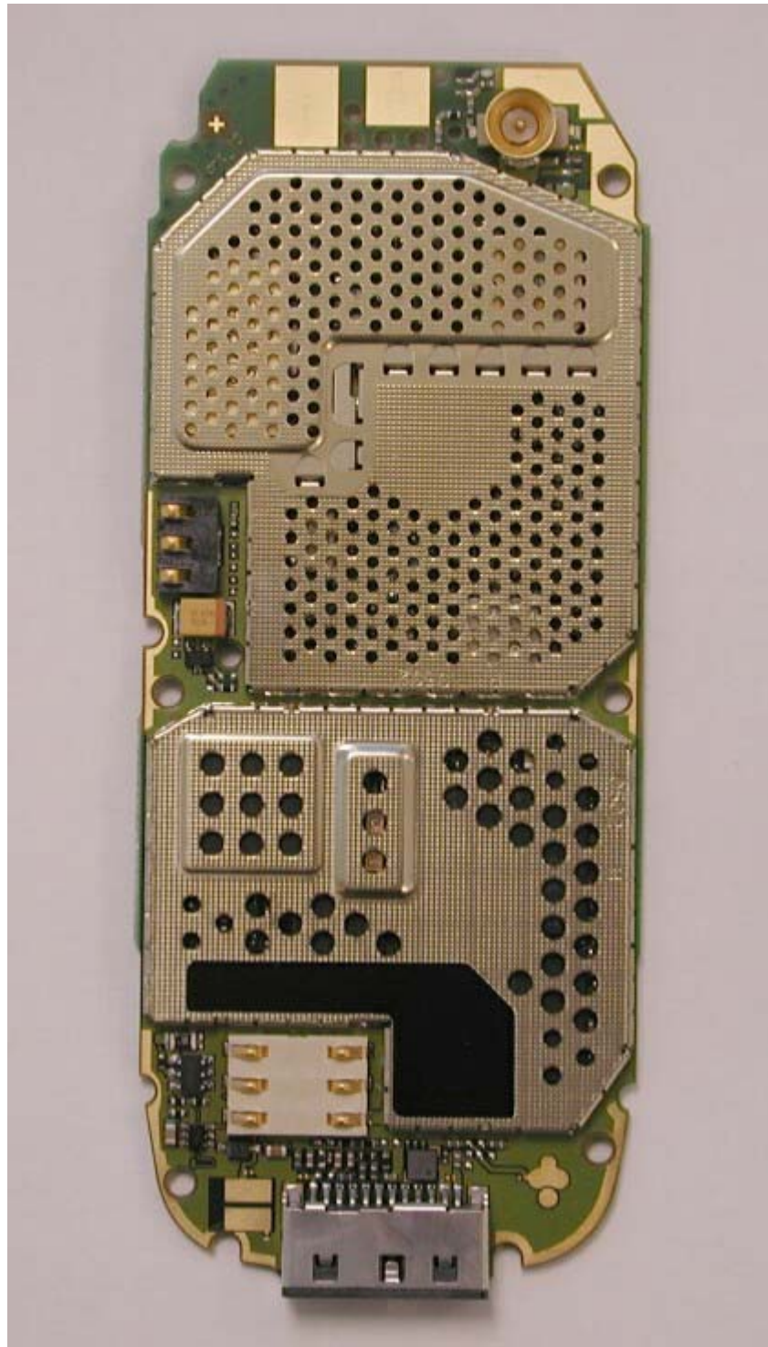
A56 Board with shielding lids, side 2
