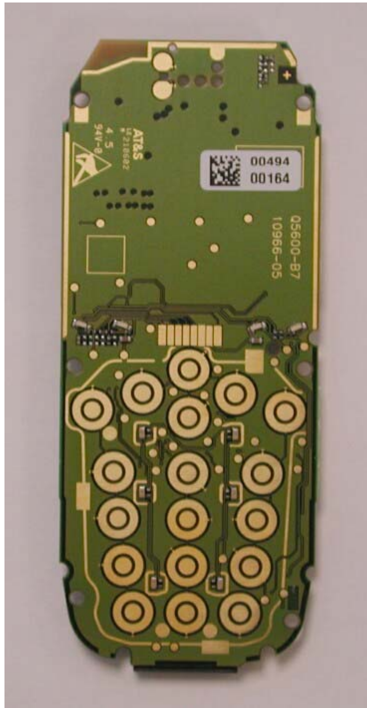
A56 Board, side 1
