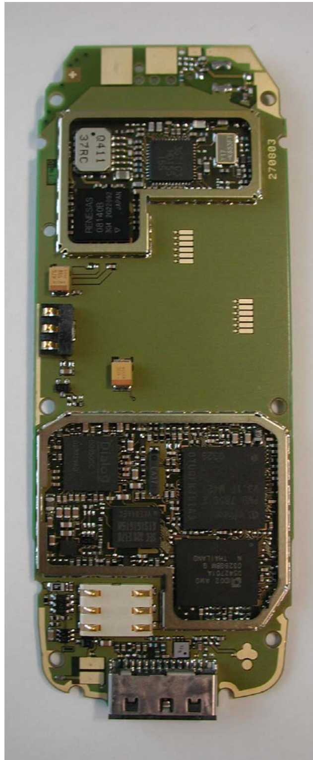
A60 Board without shield
