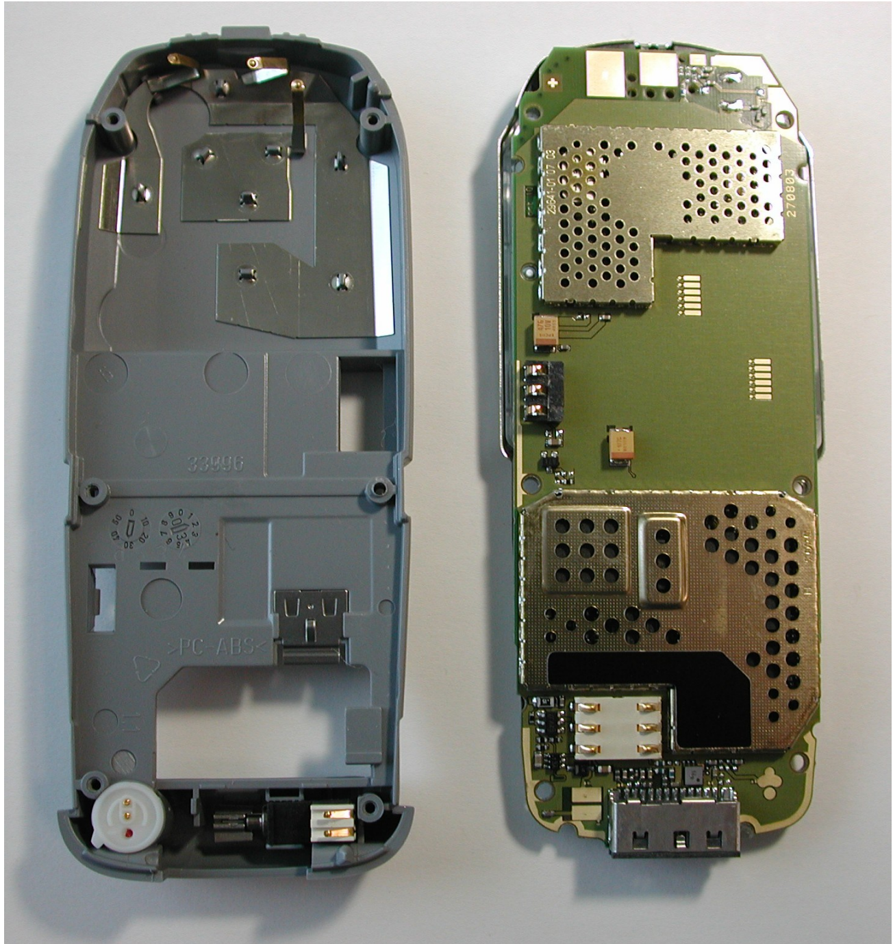
A60 Disassembly step 2
