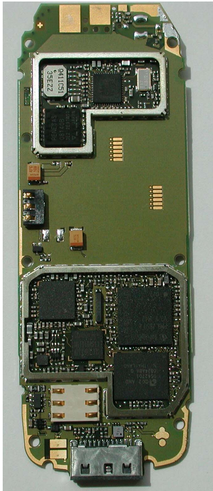
C60 Board without shield
