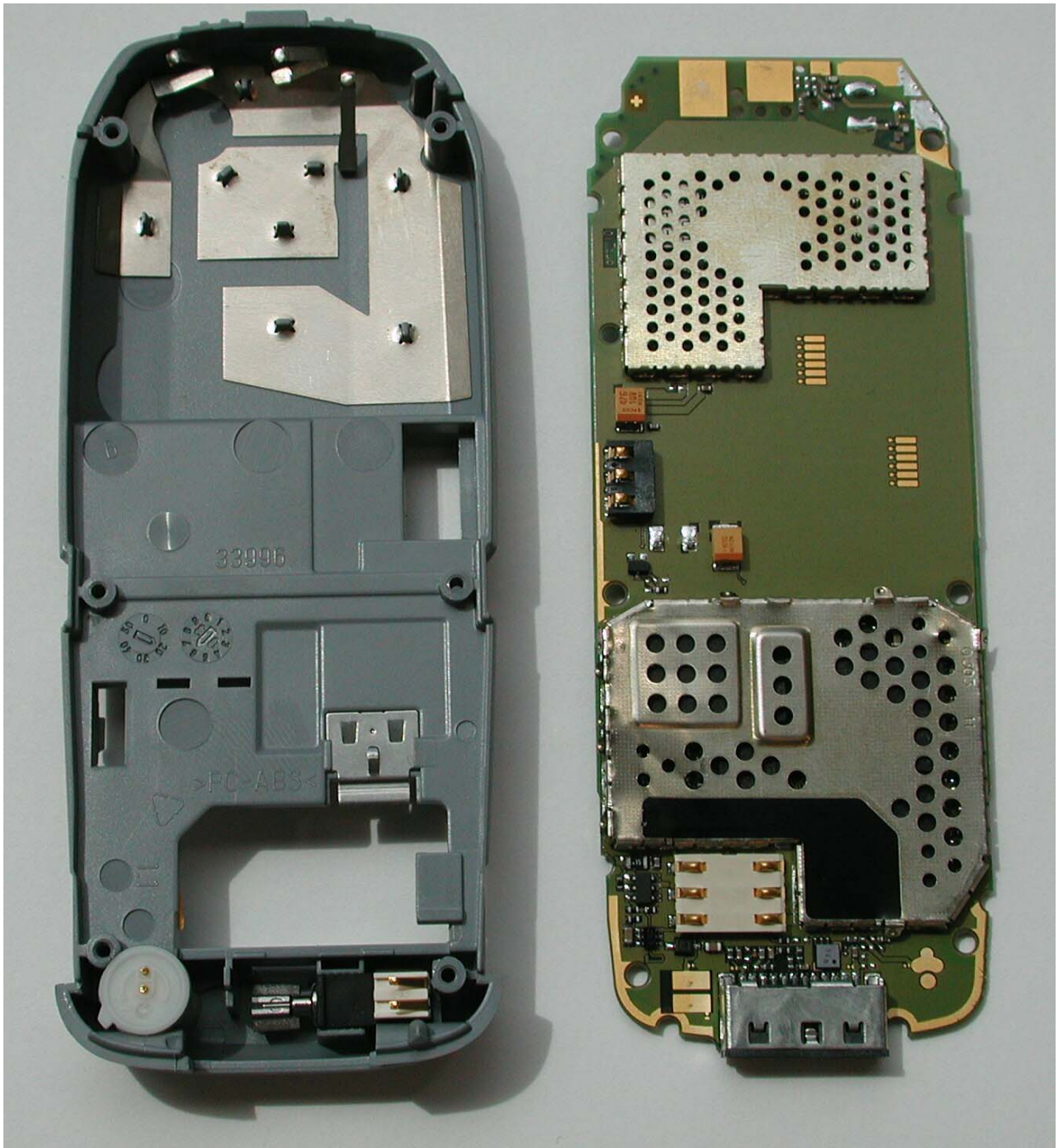
C60 Disassembly step 2
