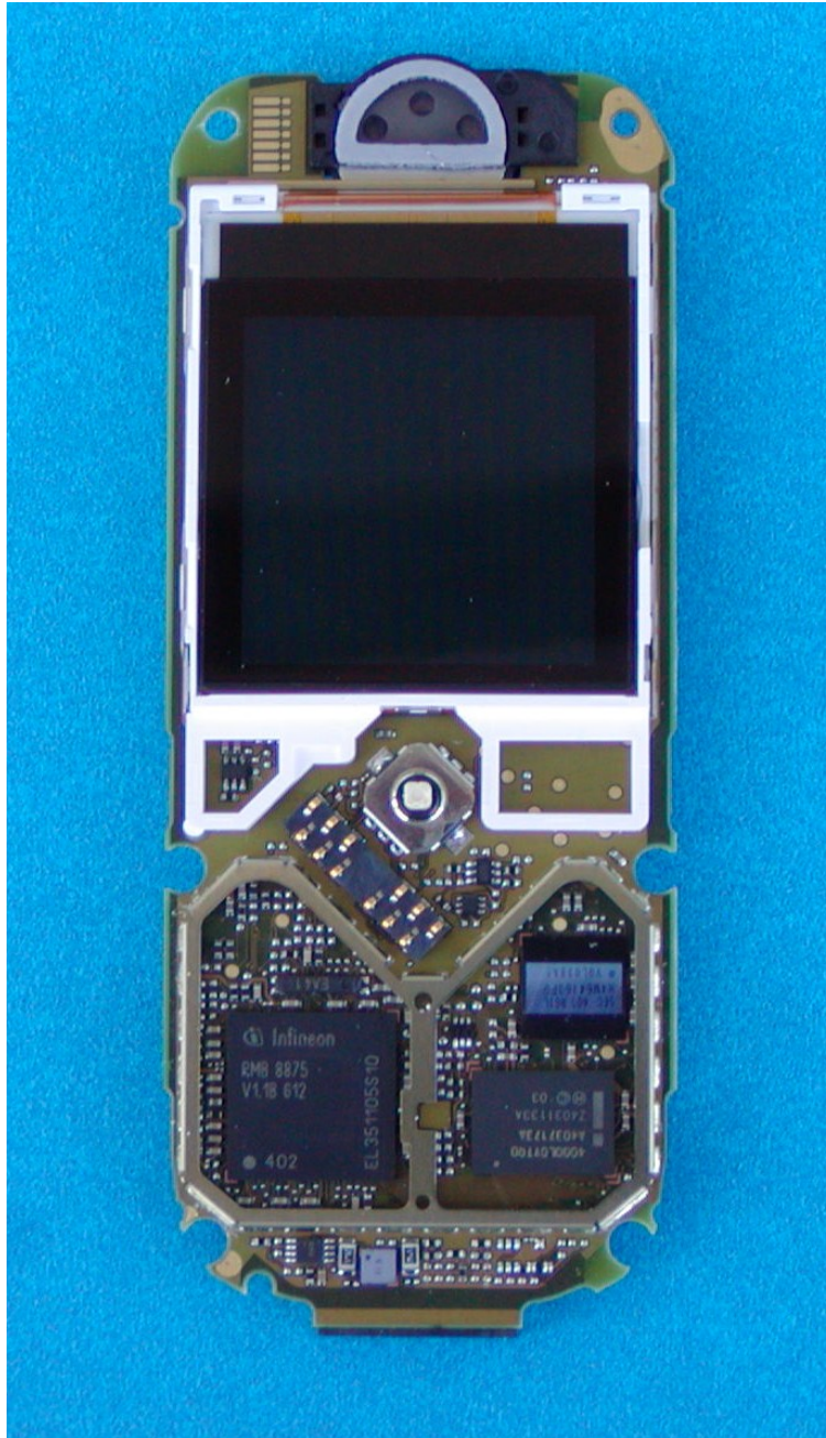
C65 PCB Front View Shields Removed
