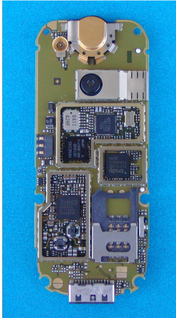
C65 PCB Rear View Shields Removed
