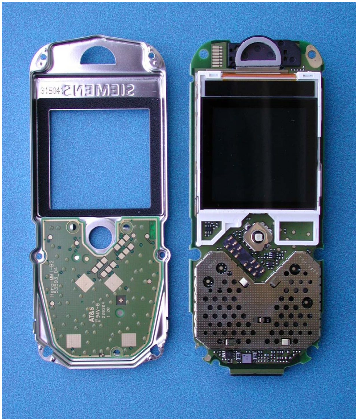
C66 Disassembly step 3
