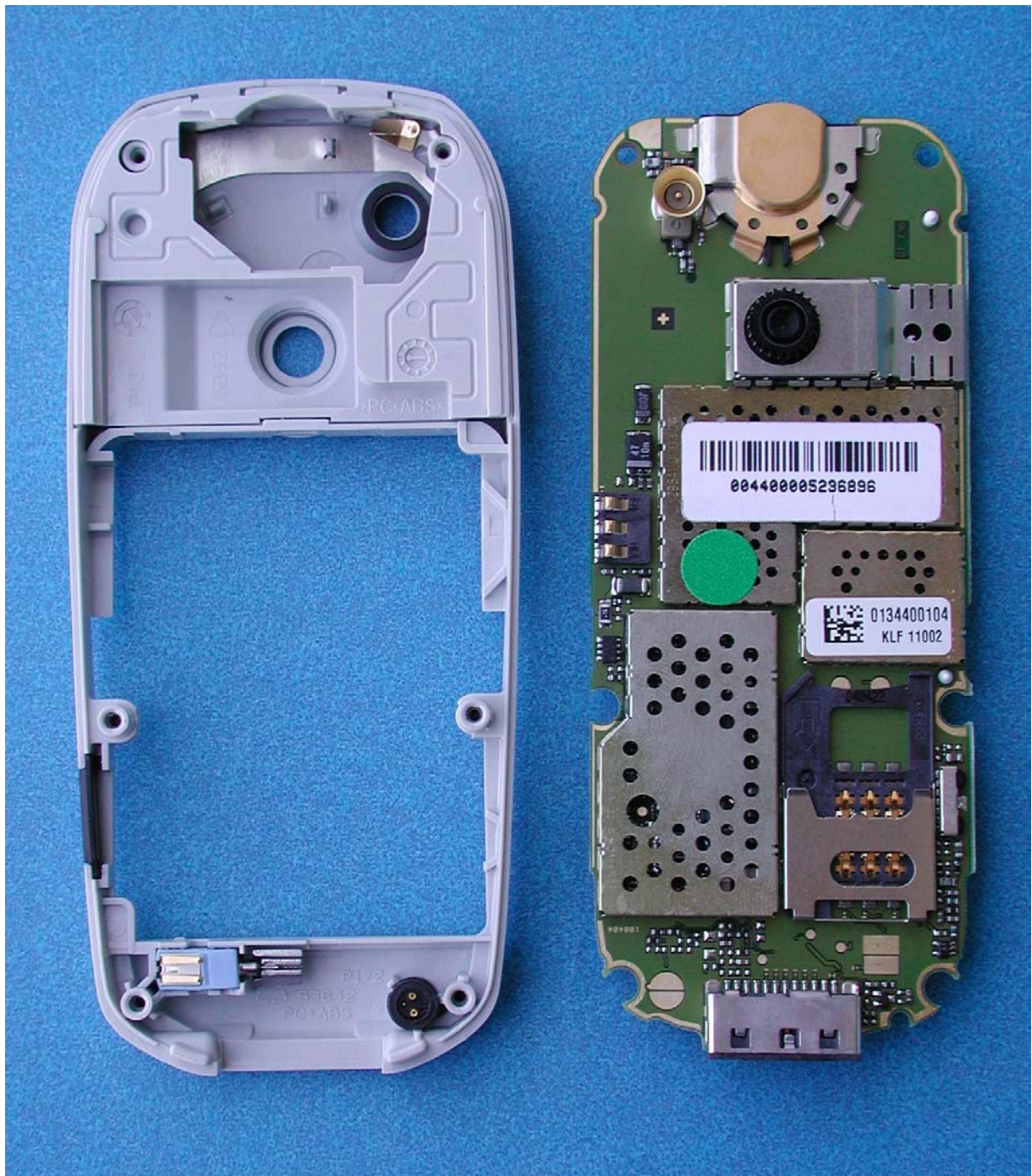
C66 Disassembly step 2
