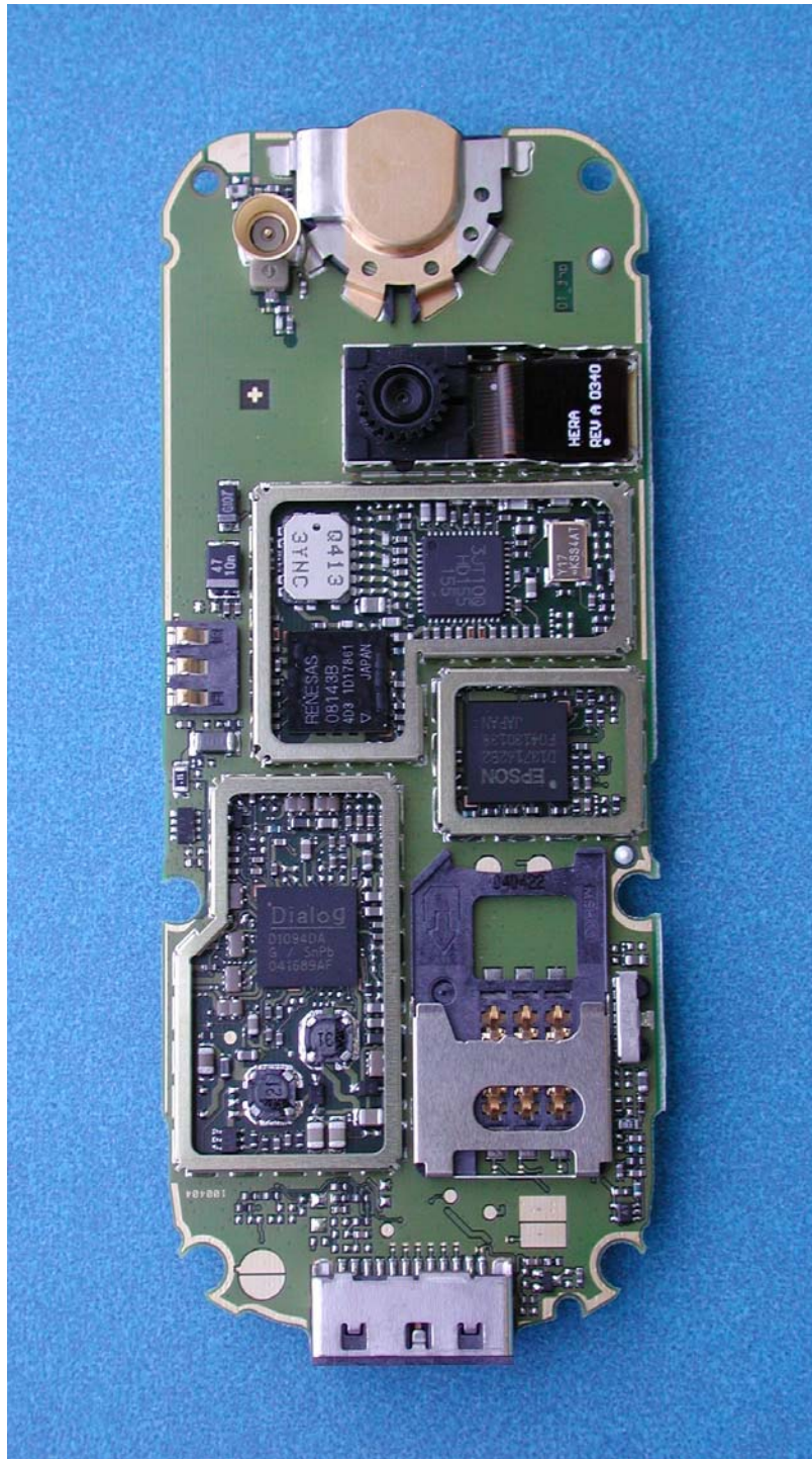
C66 PCB Rear View Shields Removed
