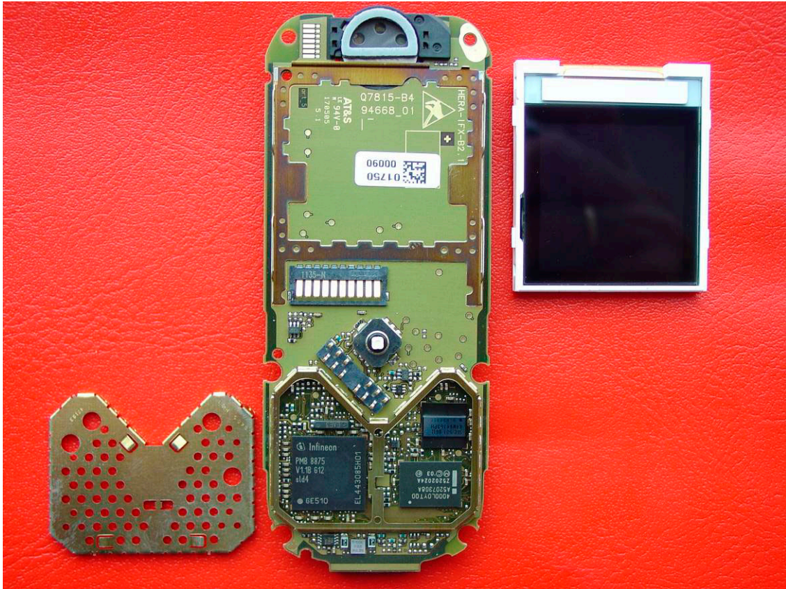
C72 Printed Circuit Board with display module and shielding lid removed.
