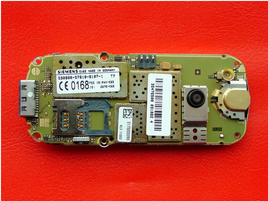
C72 Printed Circuit Board back view
