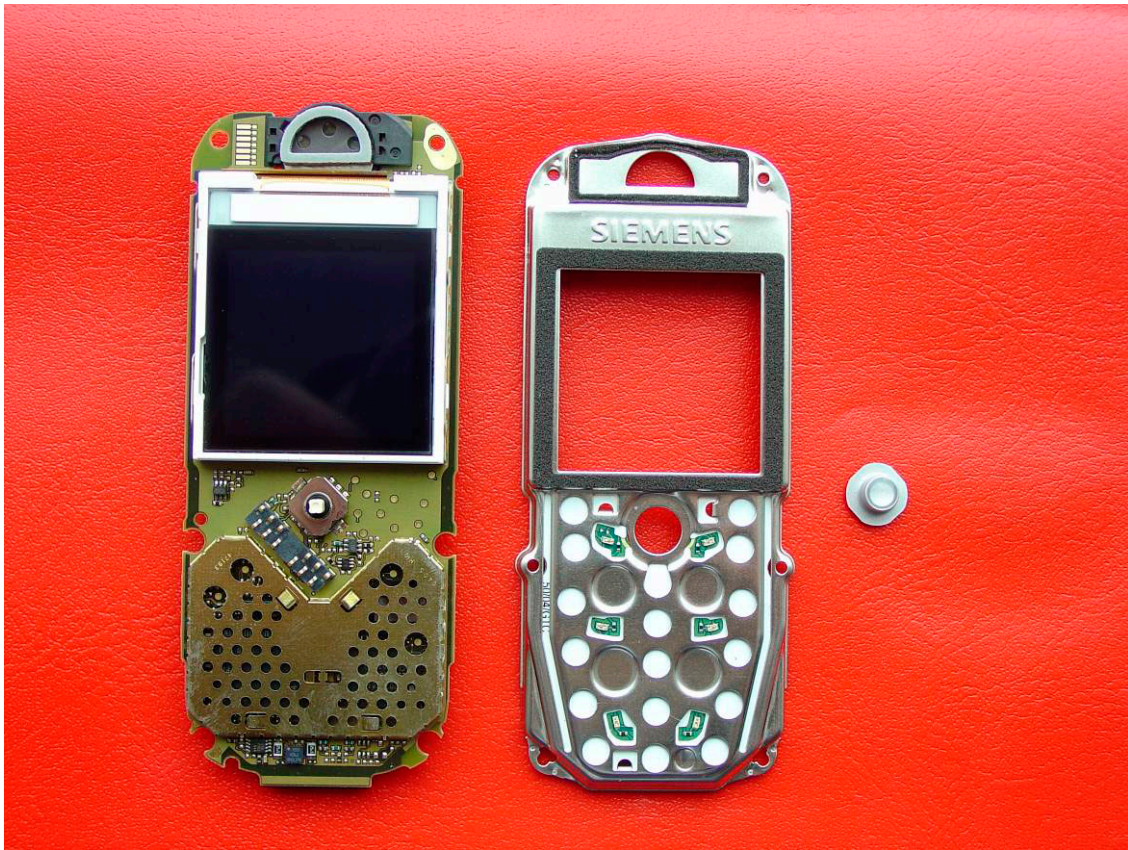
C72 Printed Circuit Board front view
