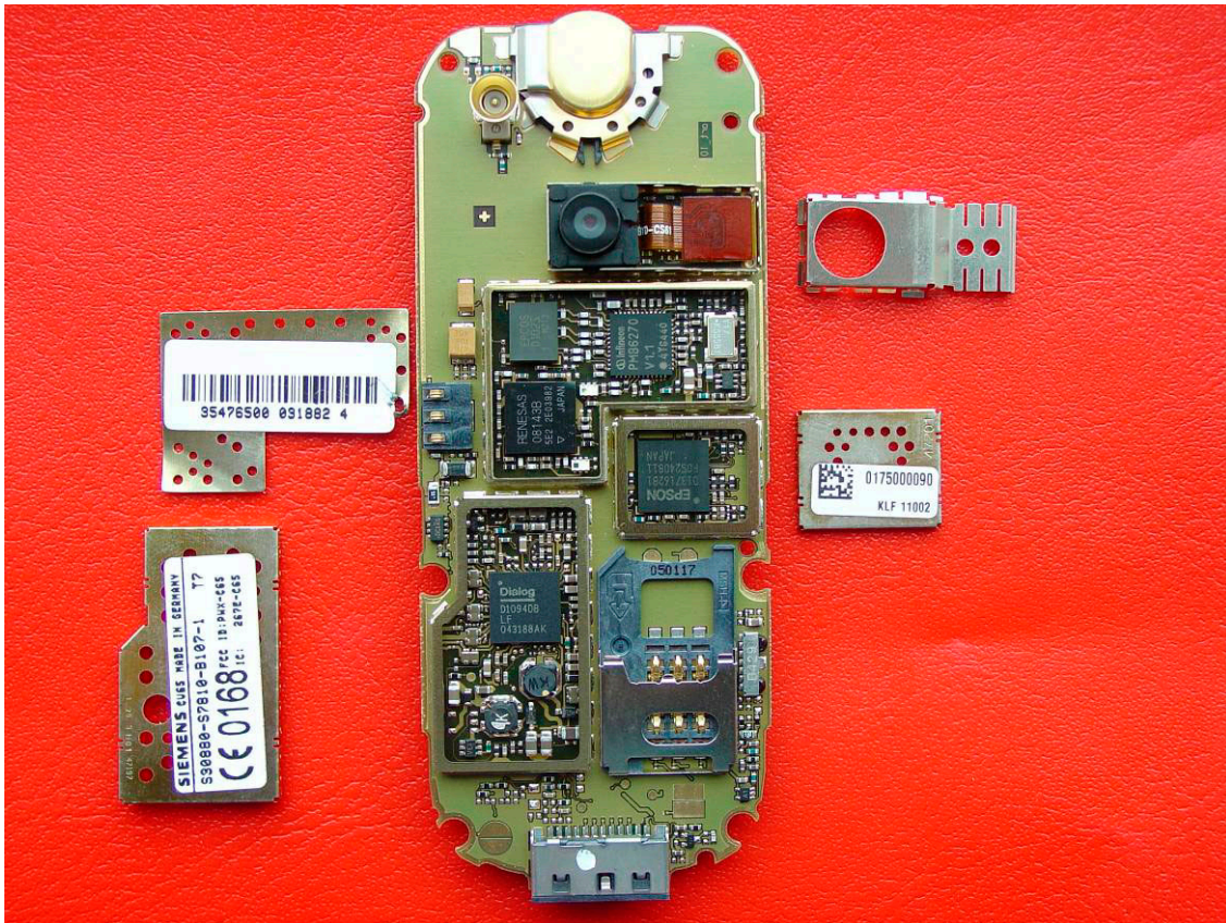
C72 Printed Circuit Boards back view with shield lid removed.
