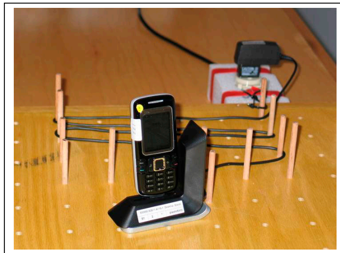
Figure 2.3 Conducted emission measurement with the travel charger US and desktop stand in the range 0.15MHz to 30 MHz.
