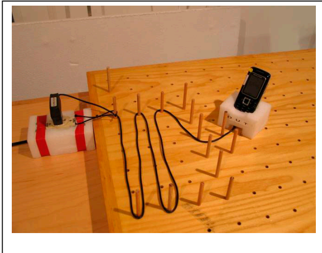
Figure 2.2 Conducted emission measurement with the travel charger in the range 0.15MHz to 30 MHz.
